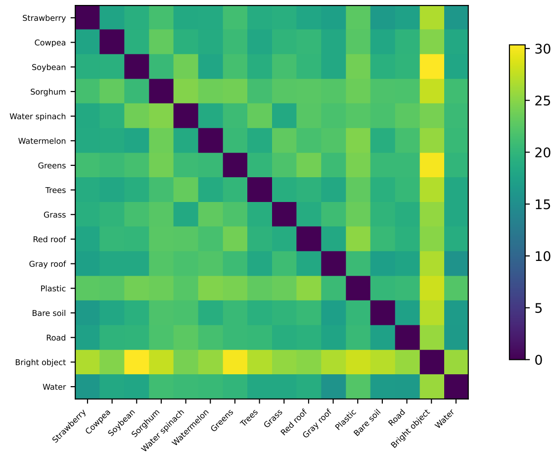
Inter-Class Distance
