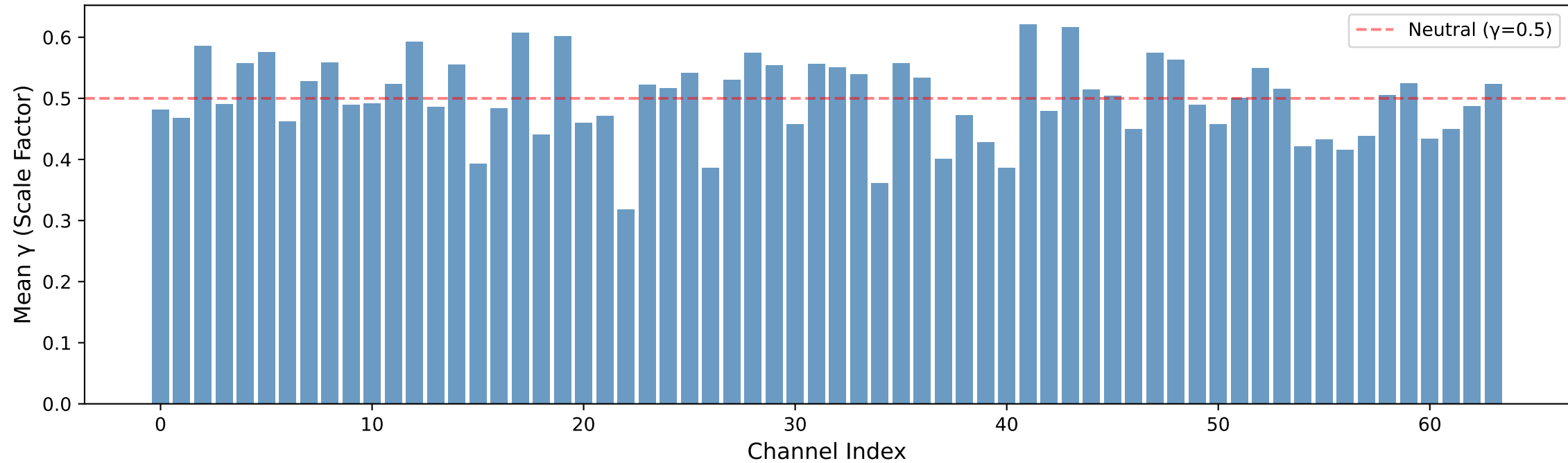
SSMRB Spectral Attention ( \gamma values) — PaviaU
