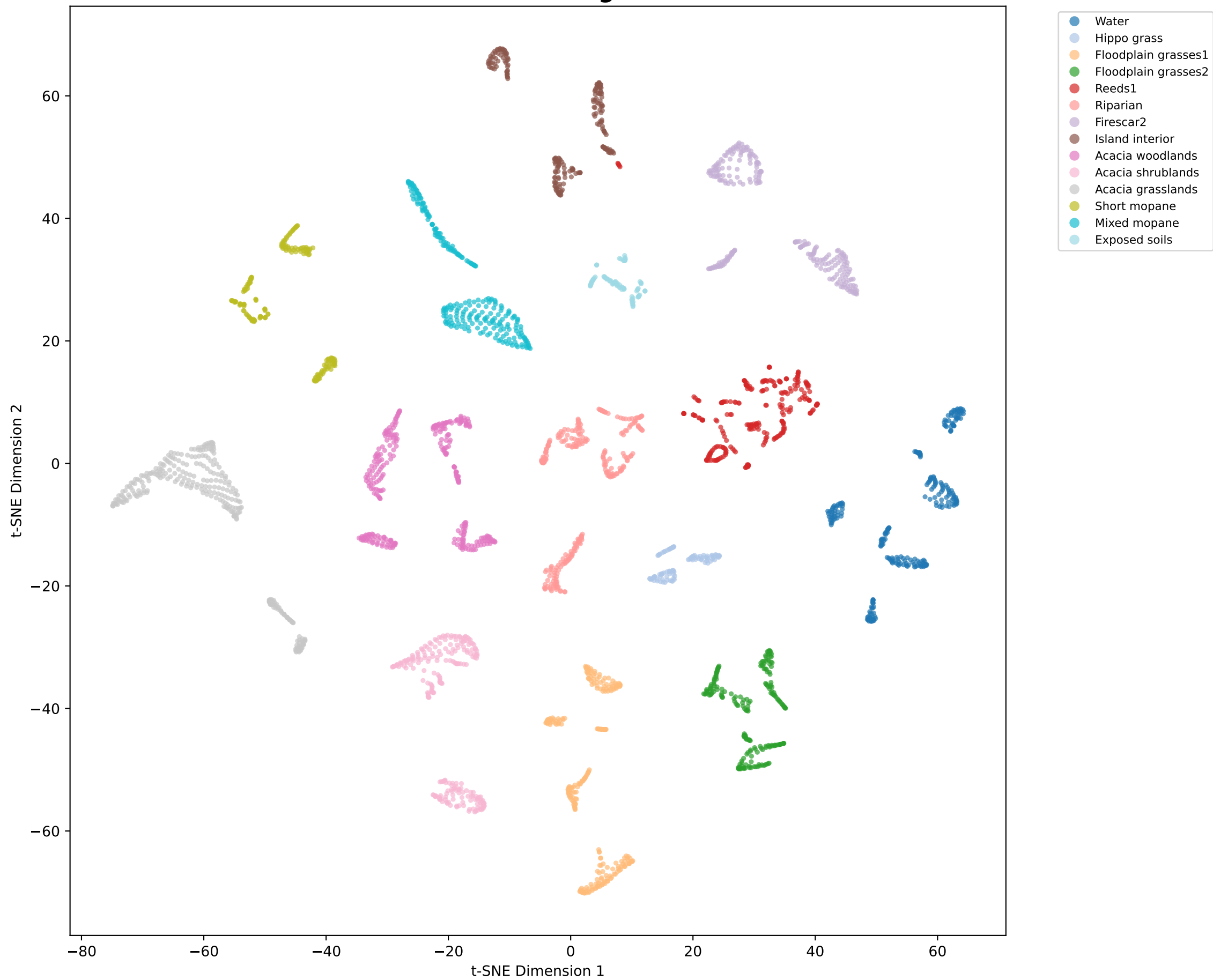
t-SNE Feature Embeddings — Botswana
