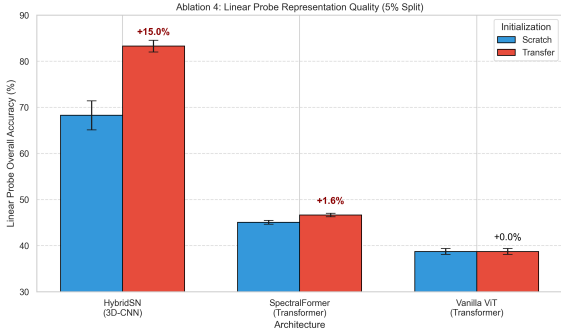
Fig. 6: Ablation 4: Linear Probe Classification (5% Split). HybridSN transfers robust, linearly separable features (+15% gain), while the evaluated transformer implementations exhibited negligible transfer gains under this annotation regime.
