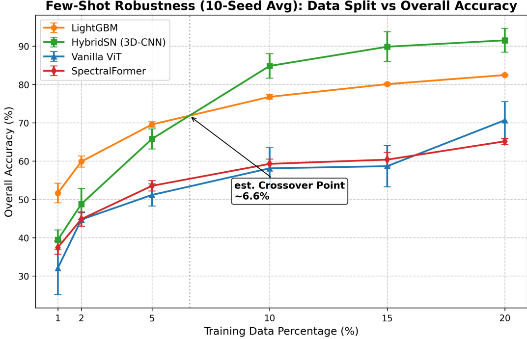
Fig. 3: Few-Shot robustness curve demonstrating the estimated crossover point at 6.6% training data, where the 3D-CNN (HybridSN) overcomes its data starvation and overtakes the pure spectral LightGBM ensemble. The newly added SpectralFormer-inspired model remains data-starved despite its inductive biases.
