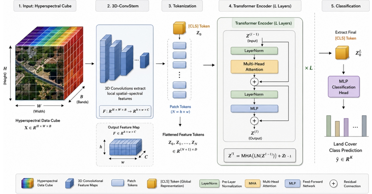
Fig. 2: The Proposed Hybrid ConvStem-Transformer Architecture. A 3D-CNN stem extracts local spatial-spectral inductive biases from the hyperspectral data cube prior to tokenization. The sequential tokens, prefixed with a global [CLS] representation, are processed by a Pre-Layer Normalization Transformer encoder. A final Multilayer Perceptron (MLP) head projects the [CLS] token to the land cover class prediction.
