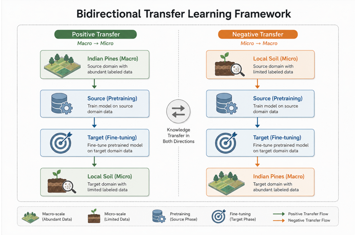
Fig. 8: Bidirectional Transfer Learning framework illustrating the tested domain hierarchies.
