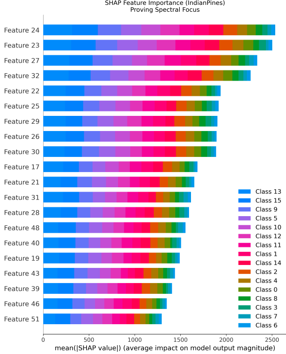
Fig. 10: Indian Pines SHAP Feature Importance, displaying prioritization even in few-shot regimes.
