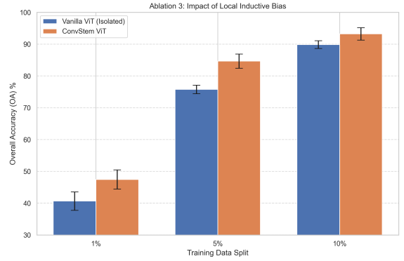
Fig. 6: Ablation 3: Impact of Local Inductive Bias. The 3D-ConvStem consistently outperforms dense spatial flattening across all splits, suggesting the importance of local feature extraction.
