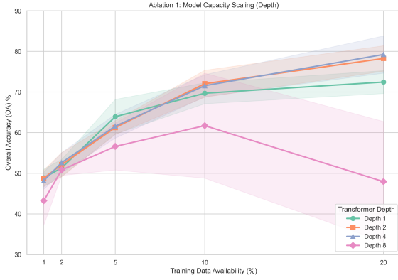
Fig. 5: Ablation 1: Model Capacity Scaling (Depth) on Indian Pines. Excessive capacity ( d = 8 ) collapses, while shallower models ( d \in \{1, 2\} ) demonstrate resilience at extreme 1-2% starvation splits.
