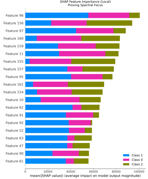
Fig. 9: Local Soil Dataset SHAP Feature Importance, prioritizing Bands 96, 156, and 97.
