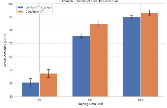
Fig. 5: Ablation 3: Impact of Local Inductive Bias. The 3D-ConvStem consistently outperforms dense spatial flattening across all splits.
