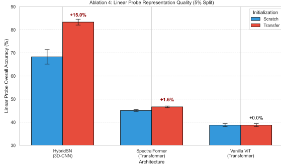
Fig. 7: Ablation 4: Linear Probe Classification (5% Split). HybridSN transfers robust, linearly separable features (+15% gain), while the evaluated transformer implementations exhibited negligible transfer gains under this annotation regime.
