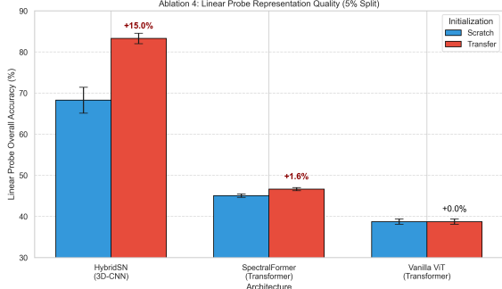
Fig. 6: Ablation 4: Linear Probe Classification (5% Split). HybridSN transfers robust, linearly separable features (+15% gain), while the evaluated transformer implementations completely fail to transfer generalized representations under this annotation regime.
