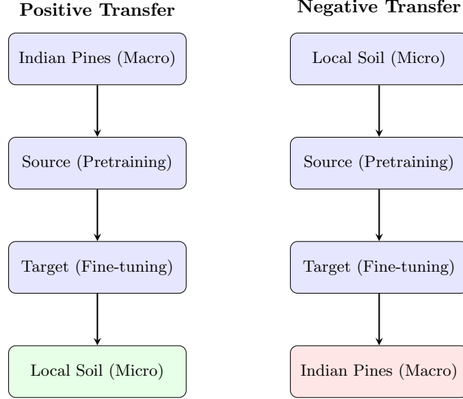
Fig. 8: Bidirectional Transfer Learning framework illustrating the tested domain hierarchies.
