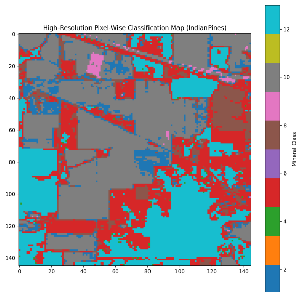
Fig. 11: Pixel-Wise Classification Map generated for the Indian Pines benchmark.
