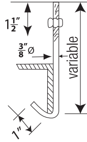
'J' Hook with nut
