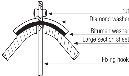
Detail of fixing point
