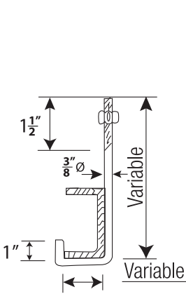
'L' Hook with nut
