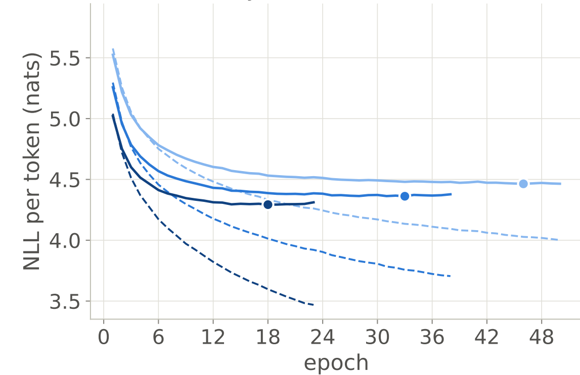
(c) LSTM, 1 layer
