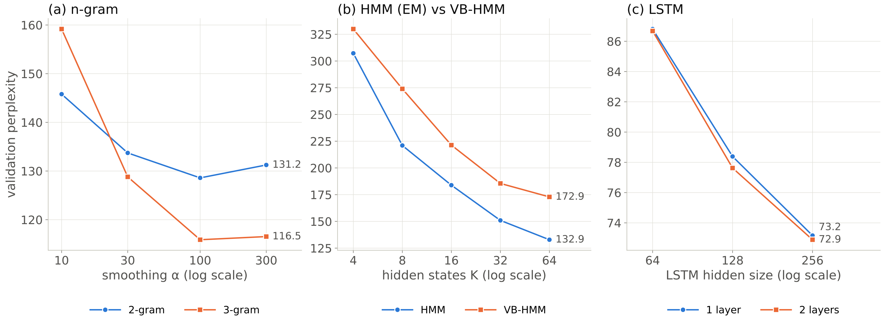
Validation perplexity by model and hyperparameter (lower is better; y-axes differ per panel)
