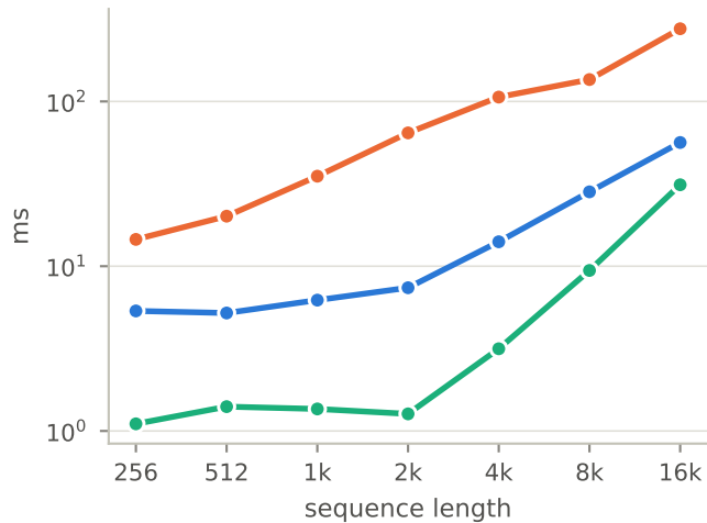
Forward latency
