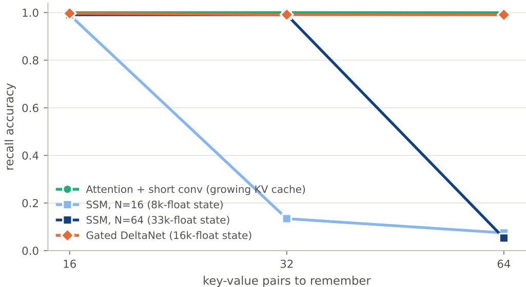
Associative recall (MQAR) vs. memory demand
