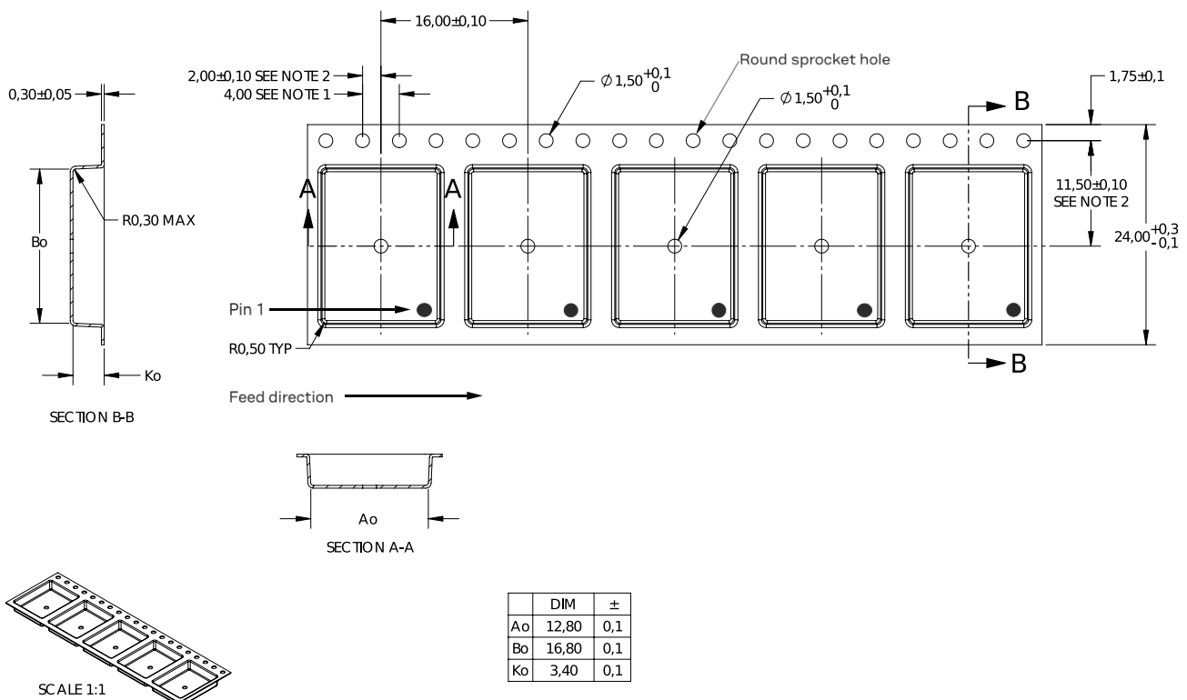
Figure 8: Dimensions (in mm) and orientation for NEO-M8P modules on tape
