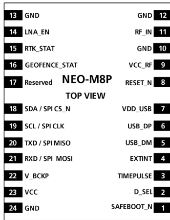
Figure 5: Pin assignment
