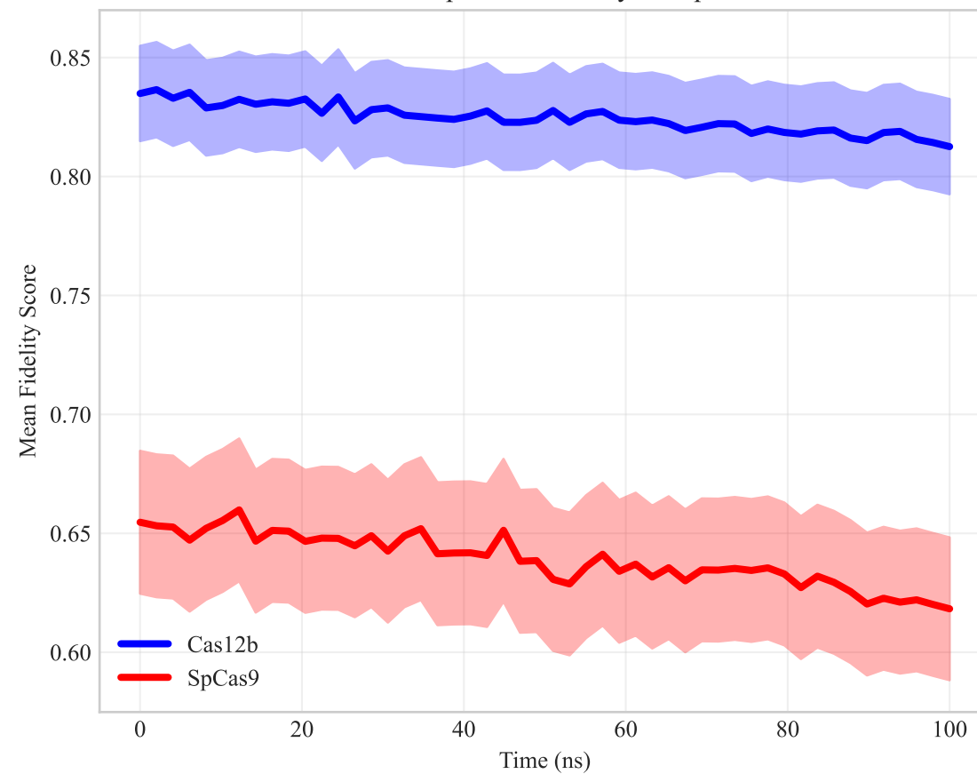
B. Time-Dependent Fidelity Comparison
