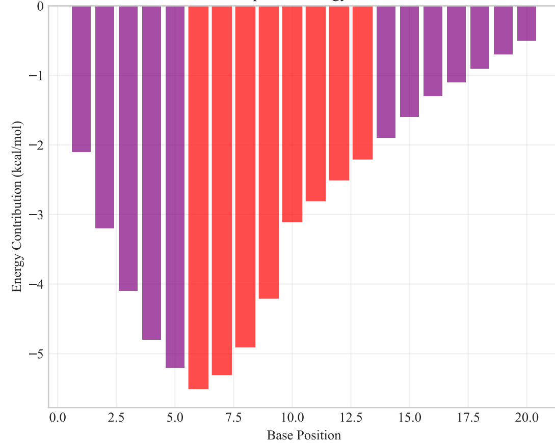
C. Position-Specific Energy Contributions
