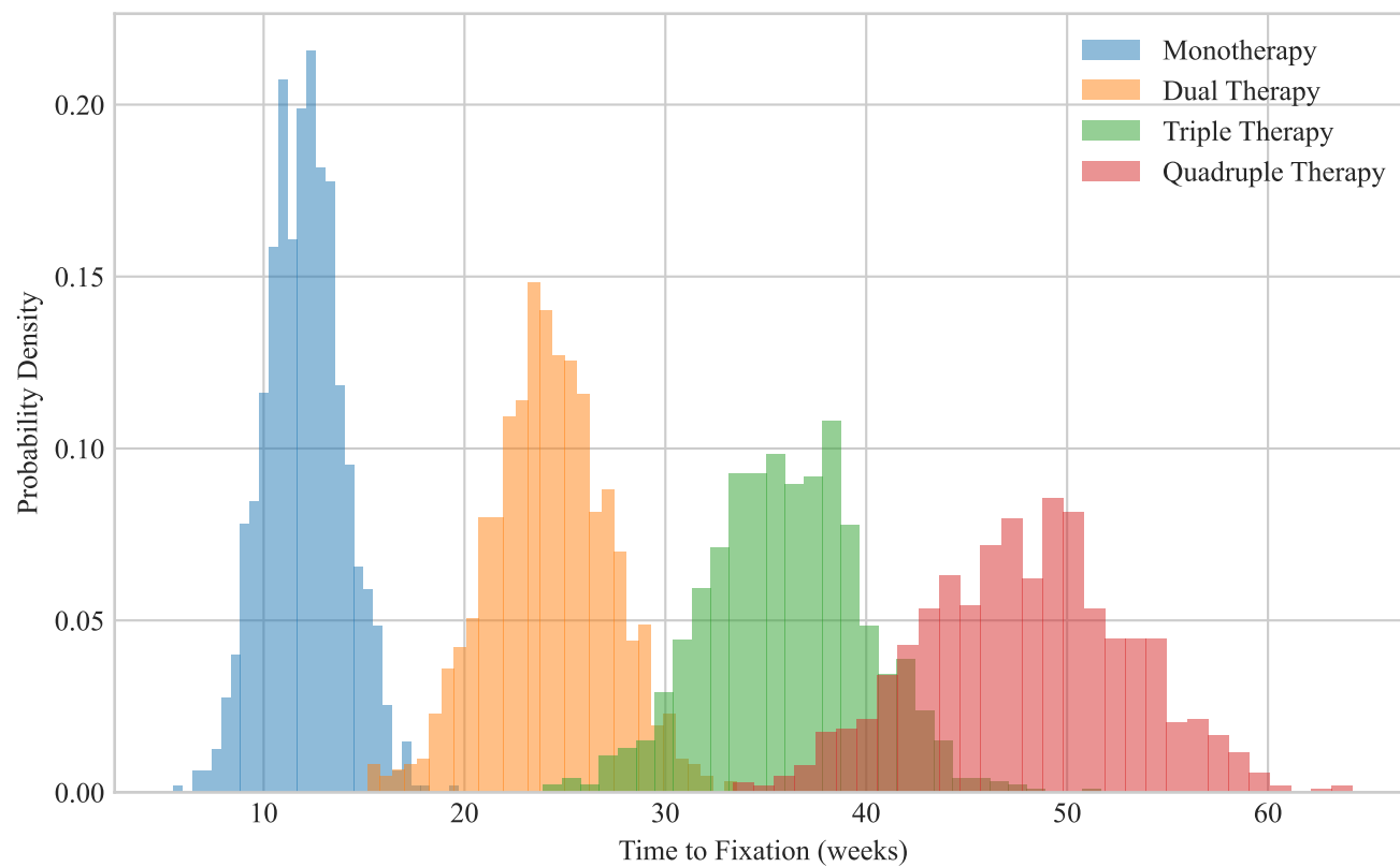
D. Fixation Time Distributions
