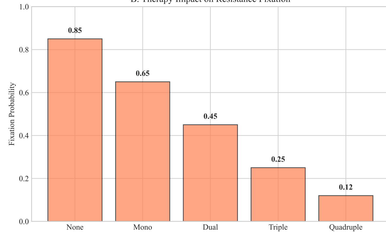
B. Therapy Impact on Resistance Fixation
