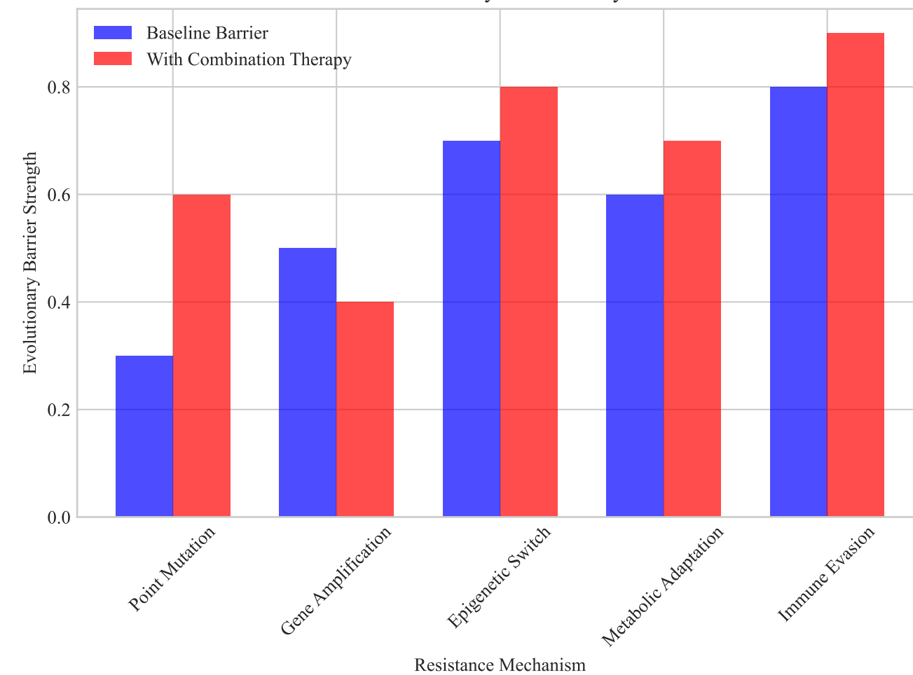
C. Evolutionary Barrier Analysis
