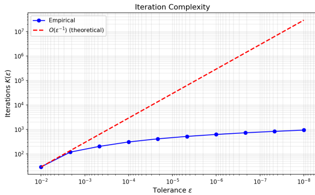
Fig. 1. Number of iterations vs. \varepsilon for PGD
