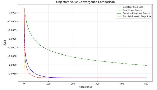
Fig. 2. Objective value f(x_k) vs. k for the different adaptative step sizes
