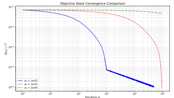
Fig. 12. \|f(x_k) - f^*\| vs iteration for several Constant Step \alpha (Tol : 10^{-6} )
