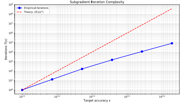
Fig. 11. Number of iterations vs. \varepsilon for the Projected Subgradient
