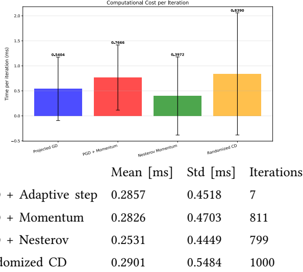
Fig. 8. Time per iteration statistics ( \varepsilon = 10^{-8} , \max\_iter = 1000 )
