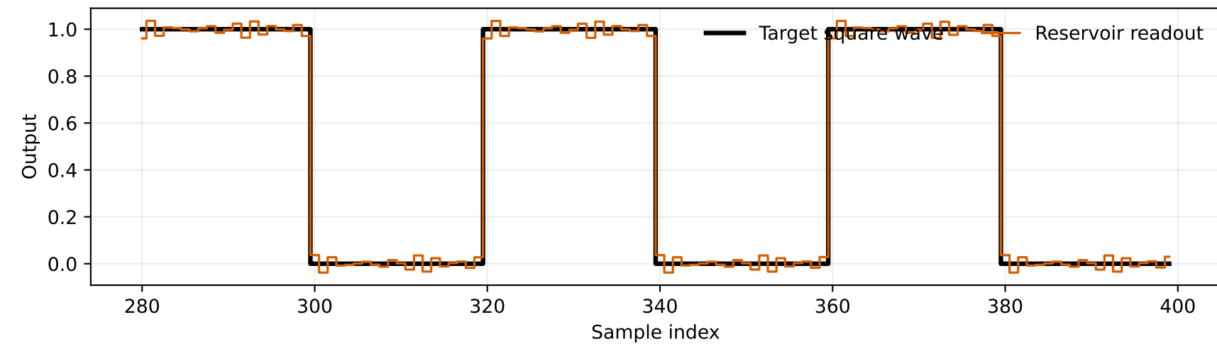
SSO 0.880 GHz — test MSE = 4.5282e-04
