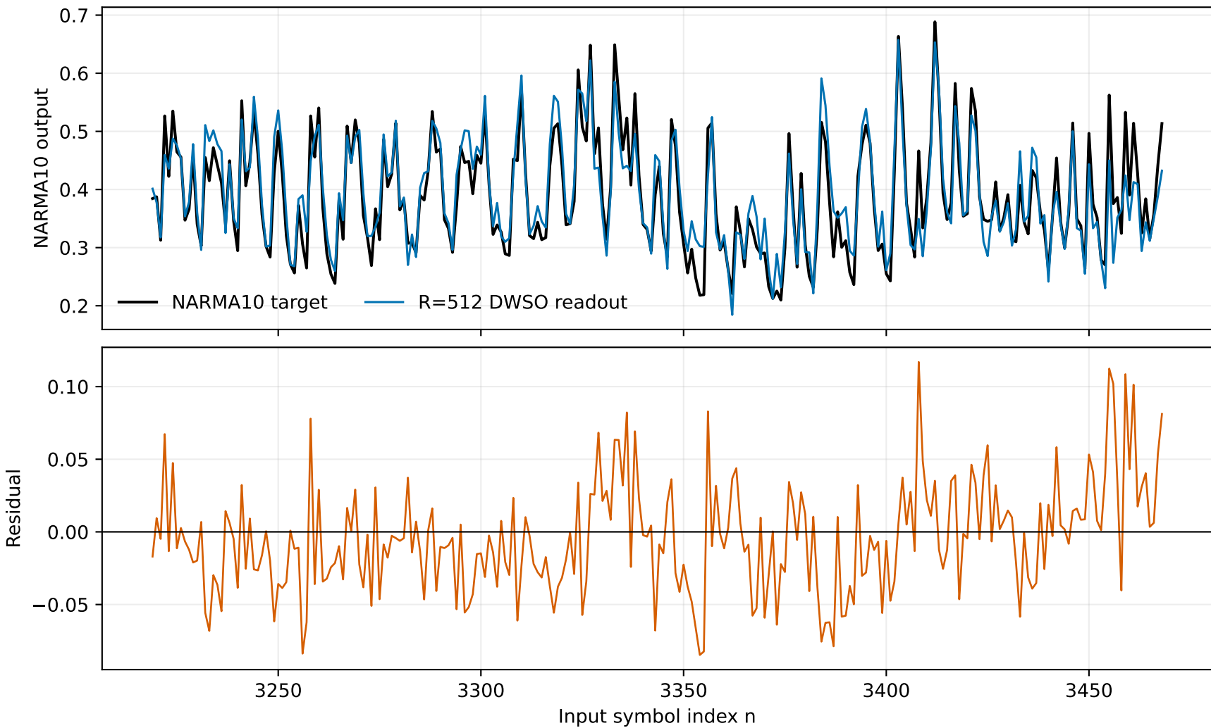
300 K DWSO, 7.3 GHz, R=512 physical-state mean test NMSE = 0.2206; MSE = 3.4656e-03
