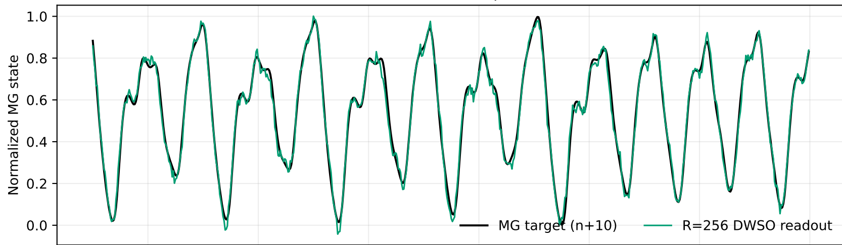
300 K DWSO, 7.3 GHz, 256-state mean — complete sealed-test MSE = 6.4653e-04
