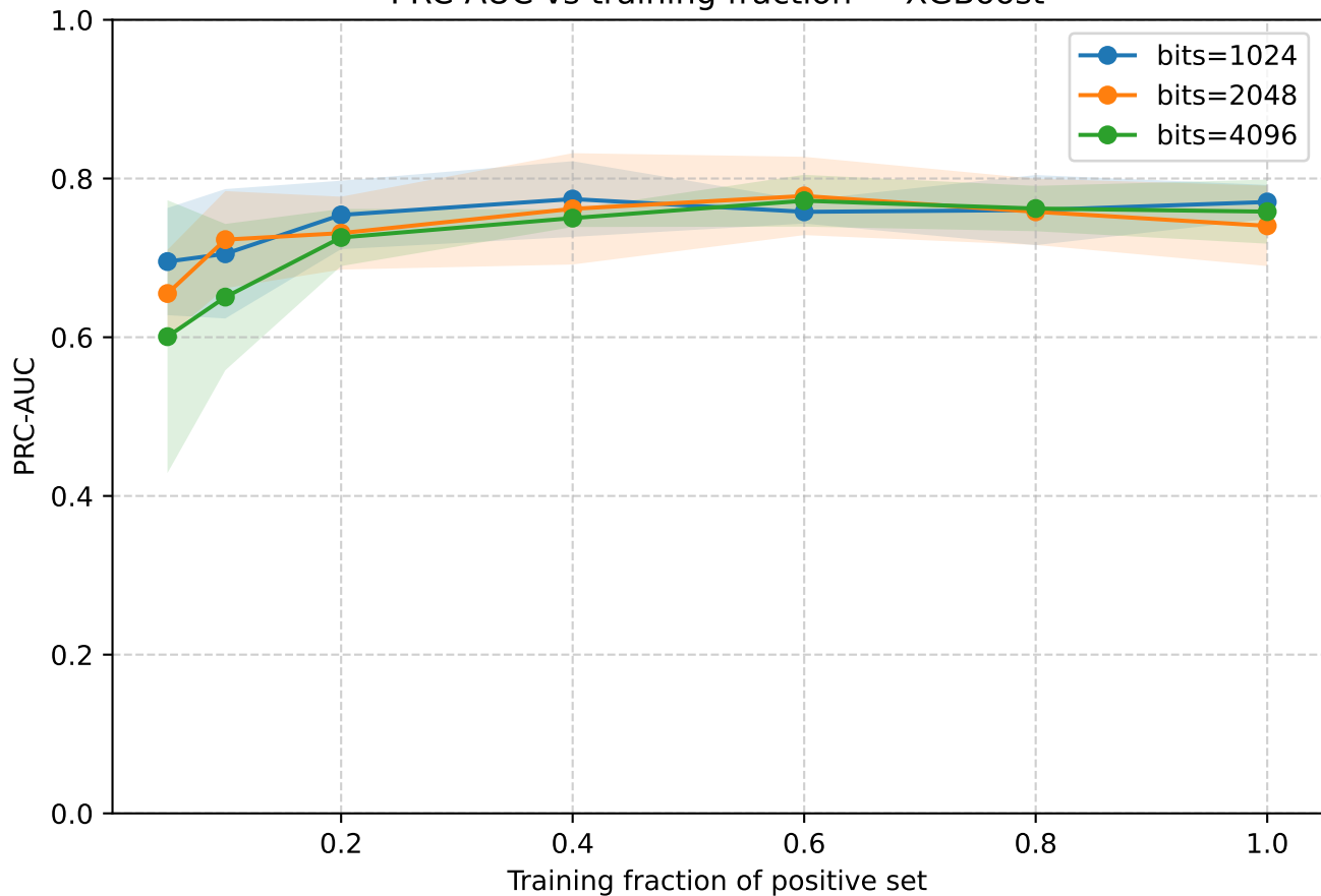
PRC-AUC vs training fraction — XGBoost
