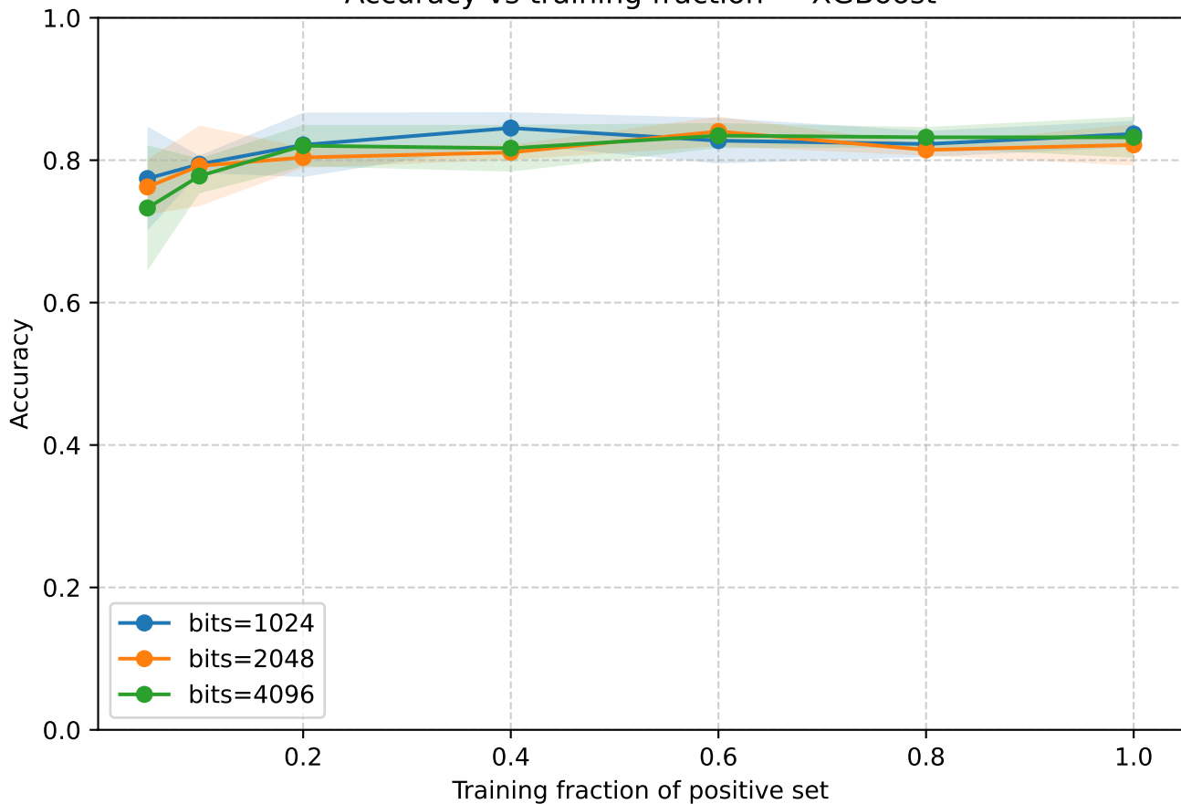
Accuracy vs training fraction — XGBoost
