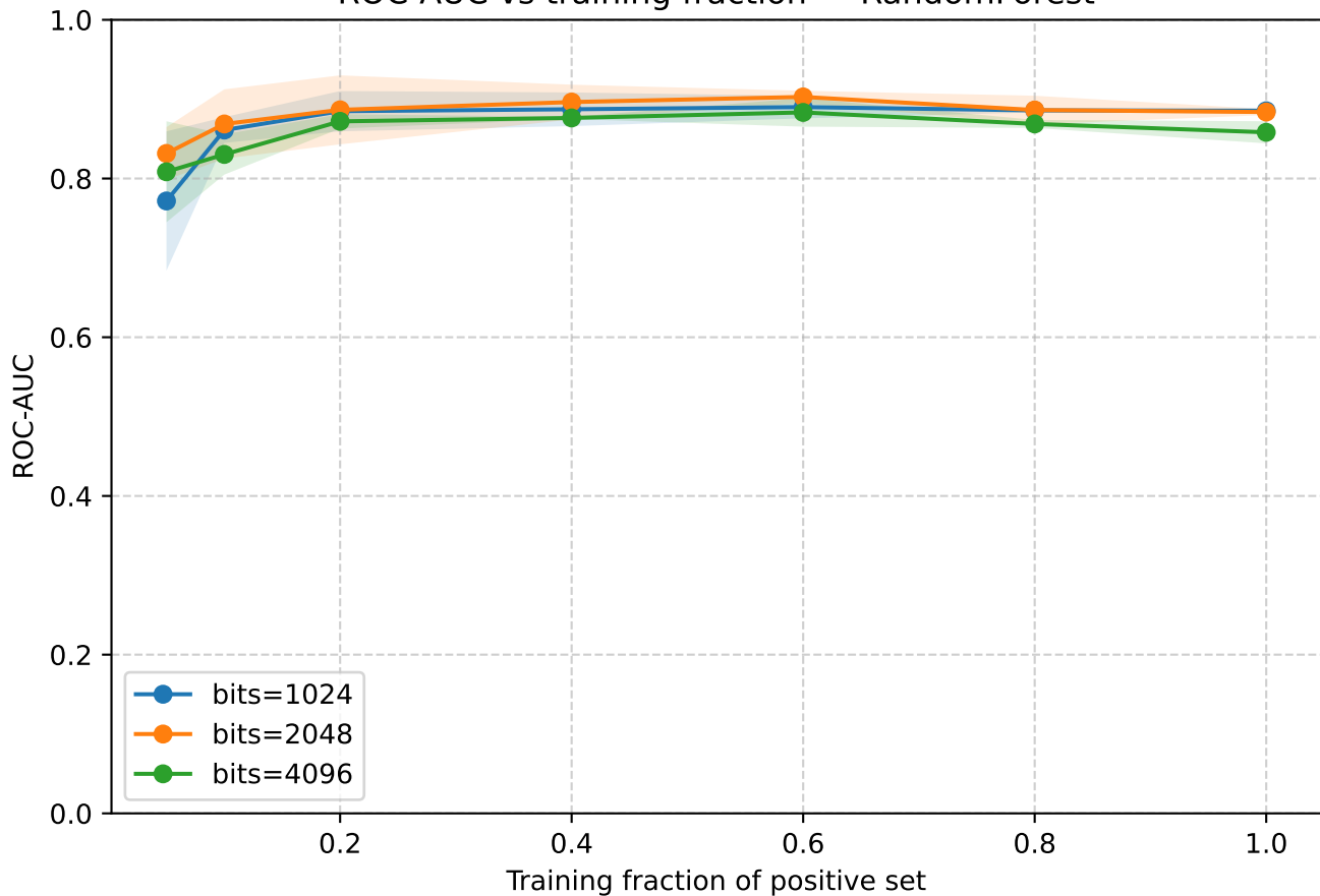
ROC-AUC vs training fraction — RandomForest
