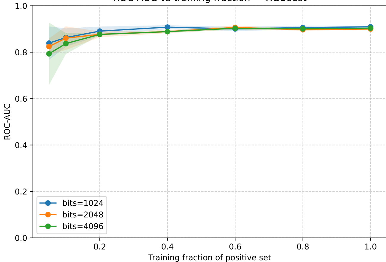
ROC-AUC vs training fraction — XGBoost
