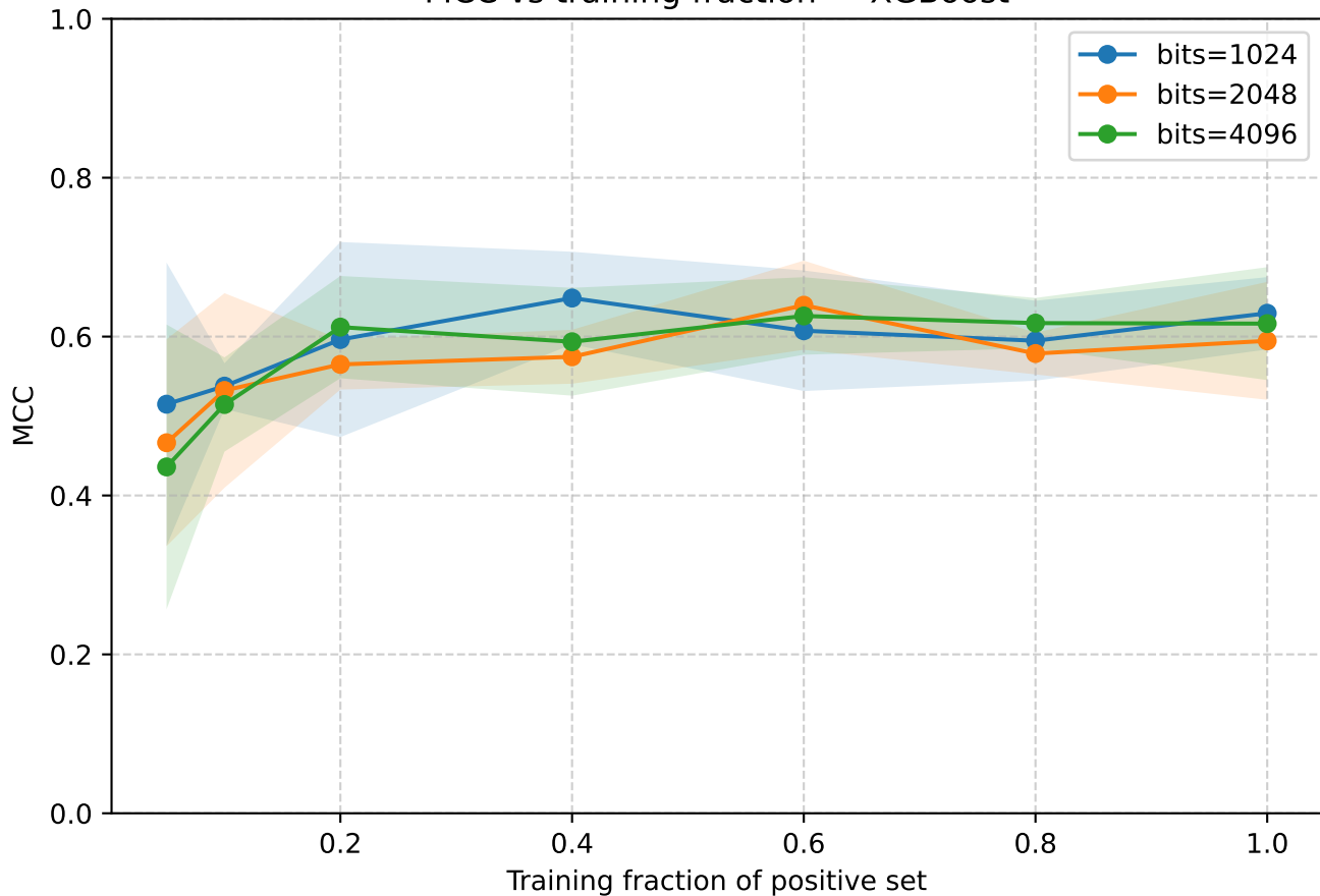
MCC vs training fraction — XGBoost
