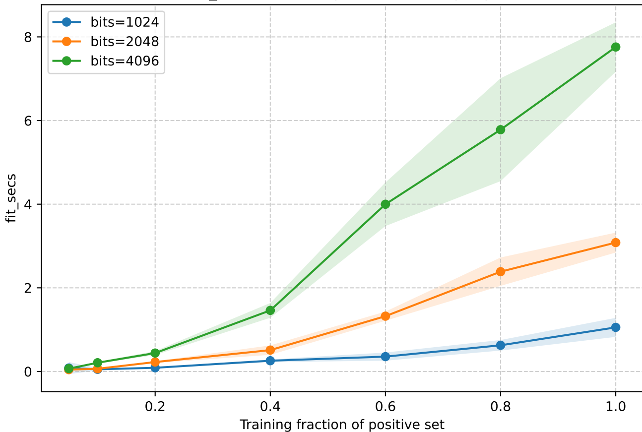
fit_secs vs training fraction — LogReg
