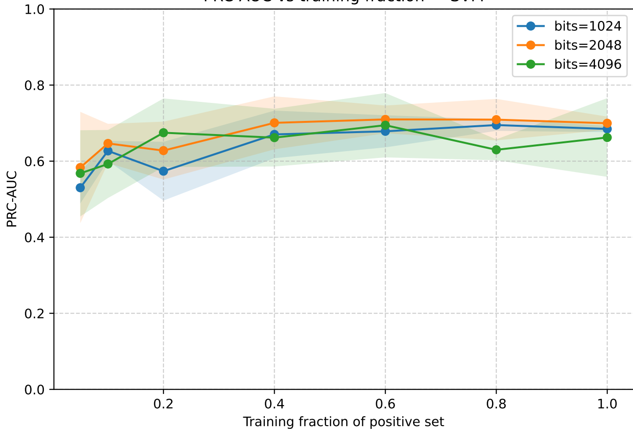
PRC-AUC vs training fraction — SVM
