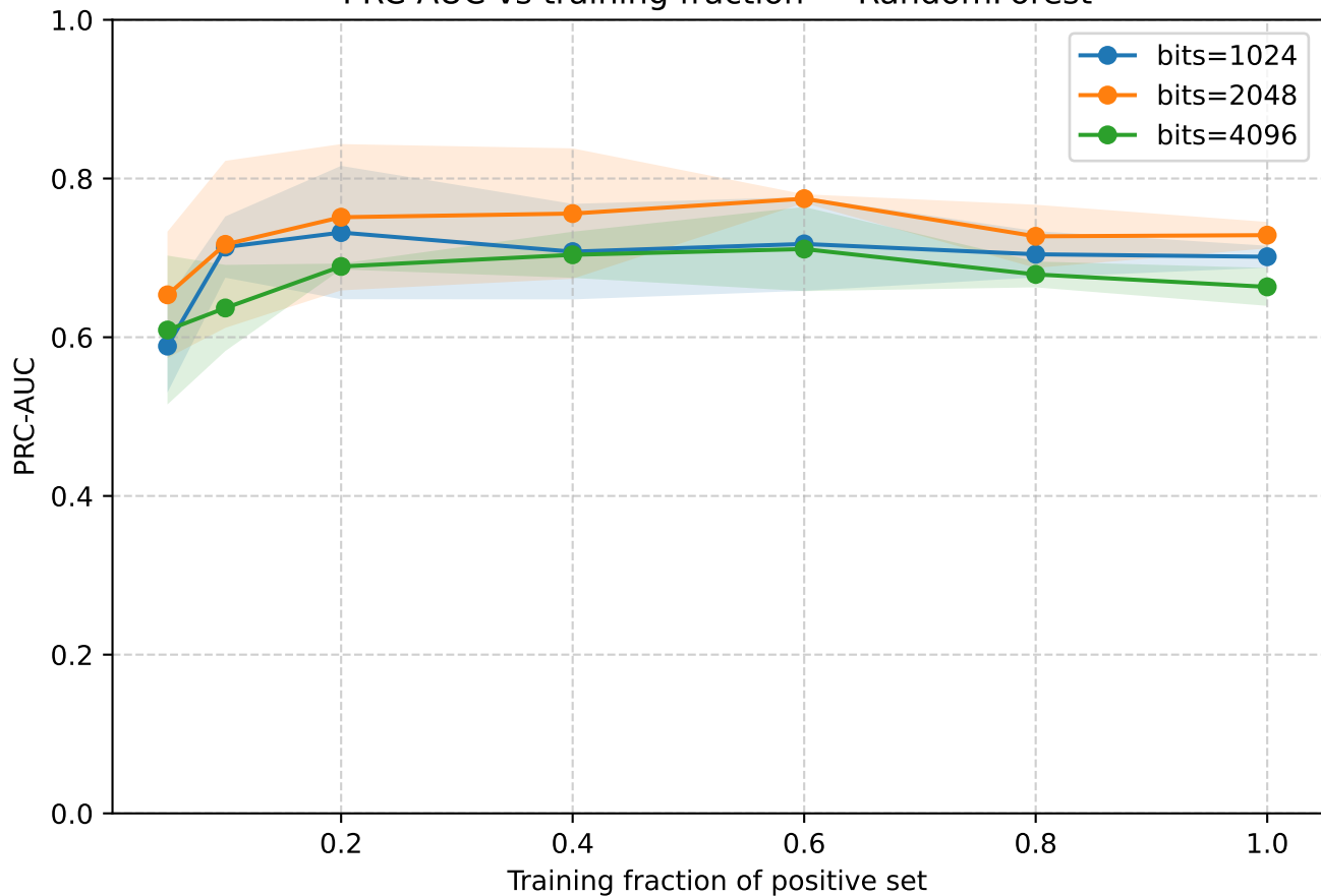
PRC-AUC vs training fraction — RandomForest
