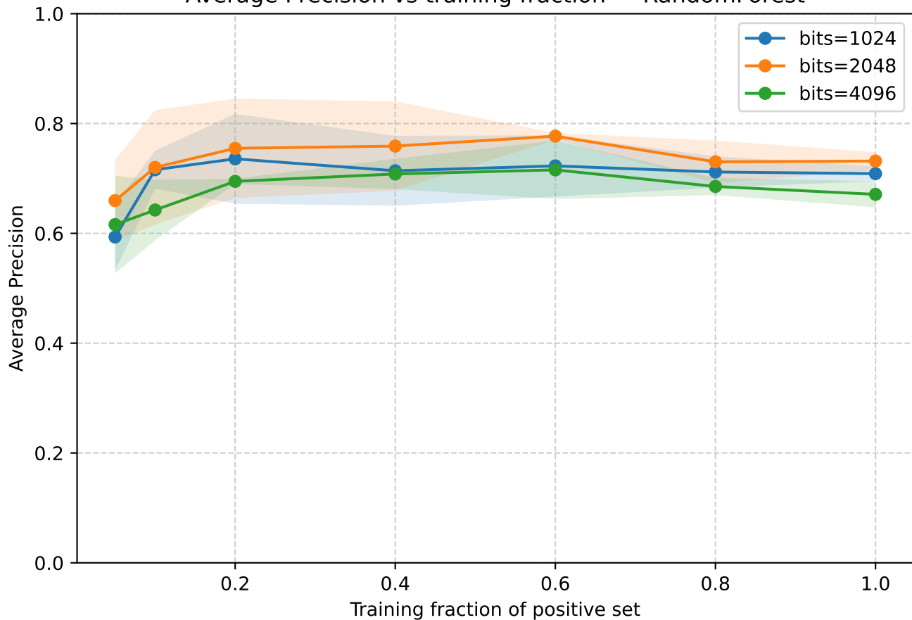
Average Precision vs training fraction — RandomForest
