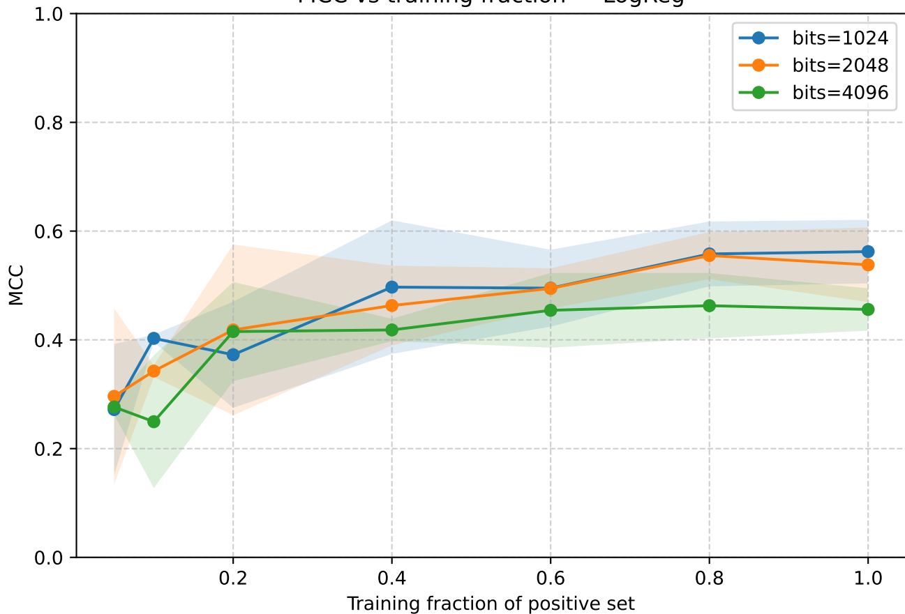
MCC vs training fraction — LogReg
