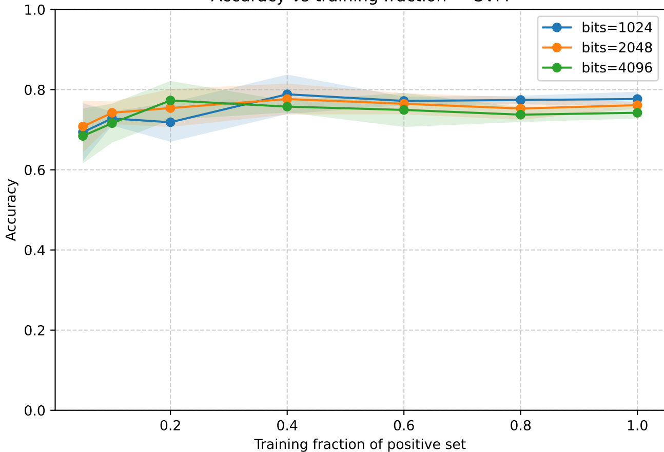
Accuracy vs training fraction — SVM
