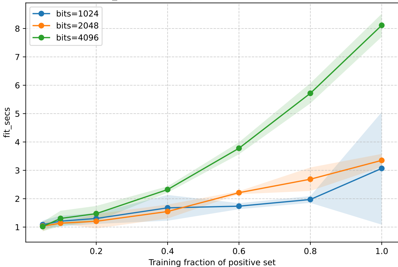
fit_secs vs training fraction — RandomForest
