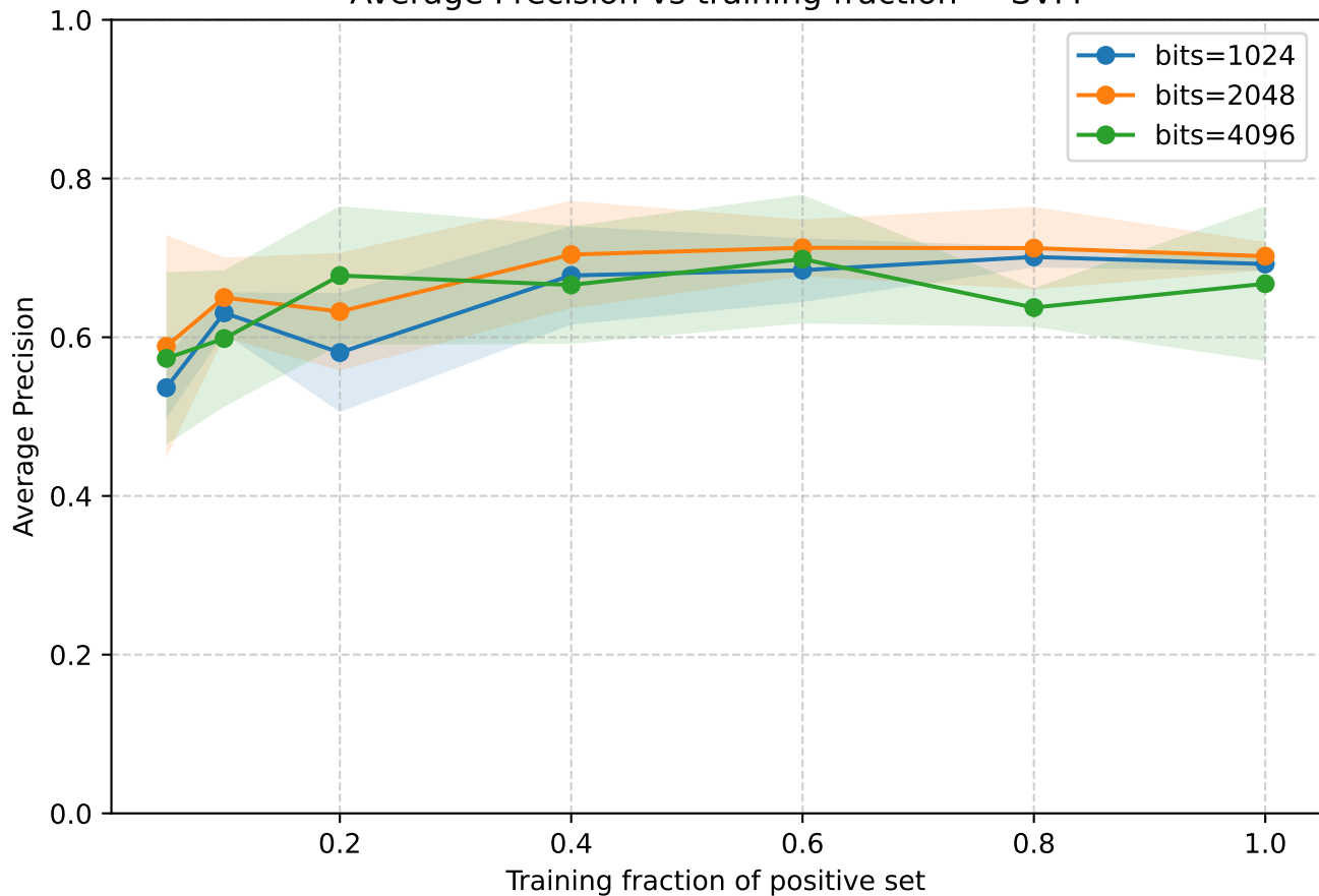
Average Precision vs training fraction — SVM
