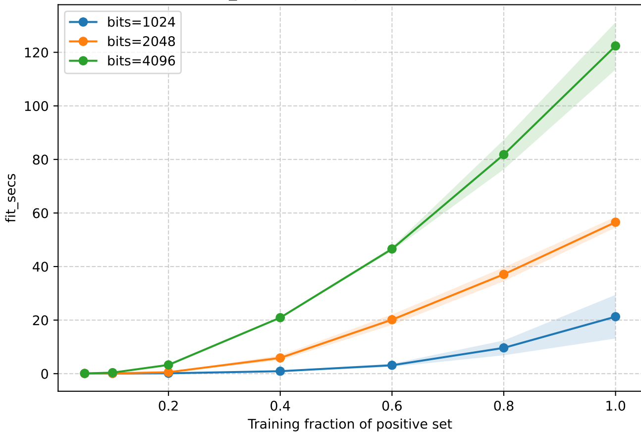
fit_secs vs training fraction — SVM
