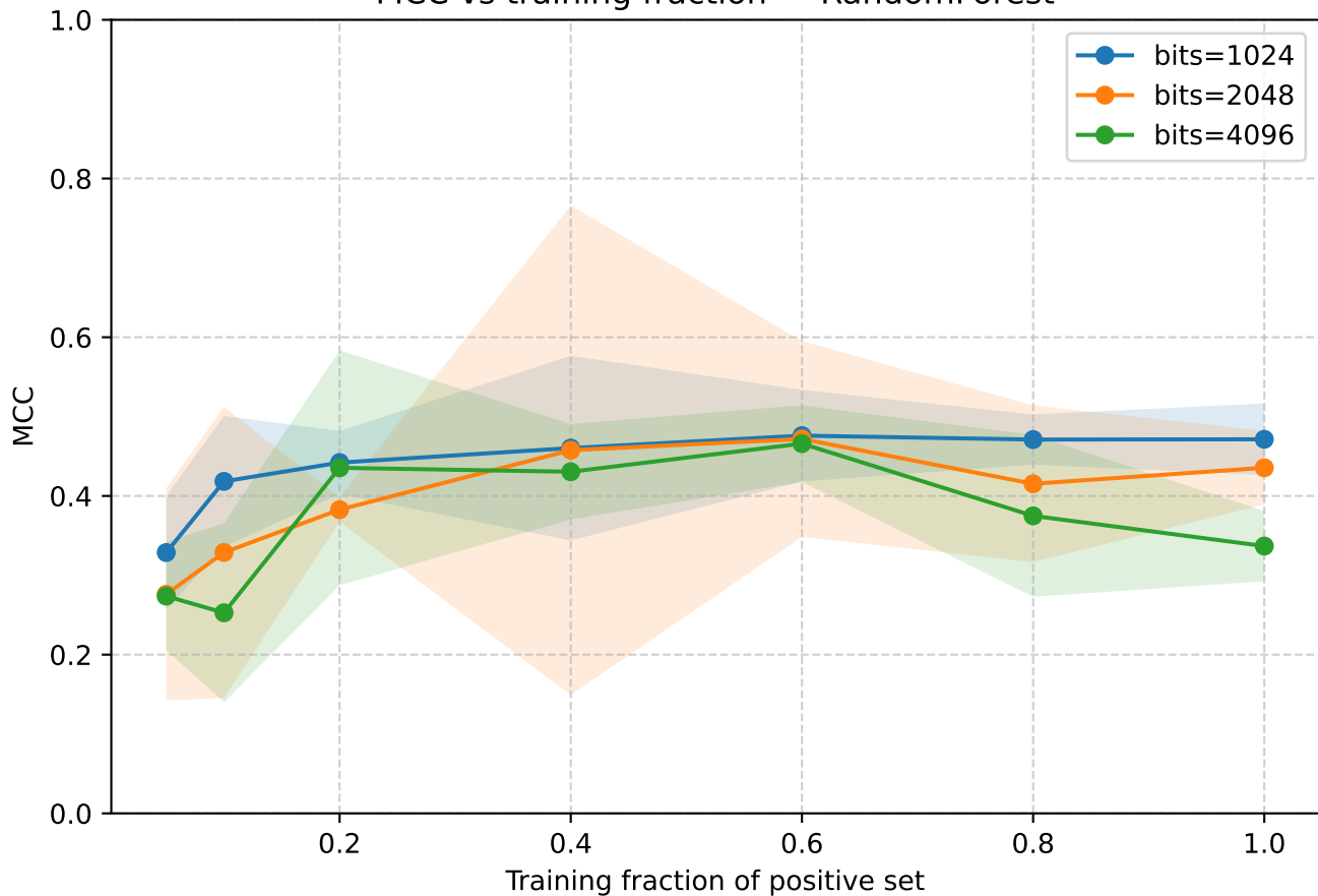
MCC vs training fraction — RandomForest
