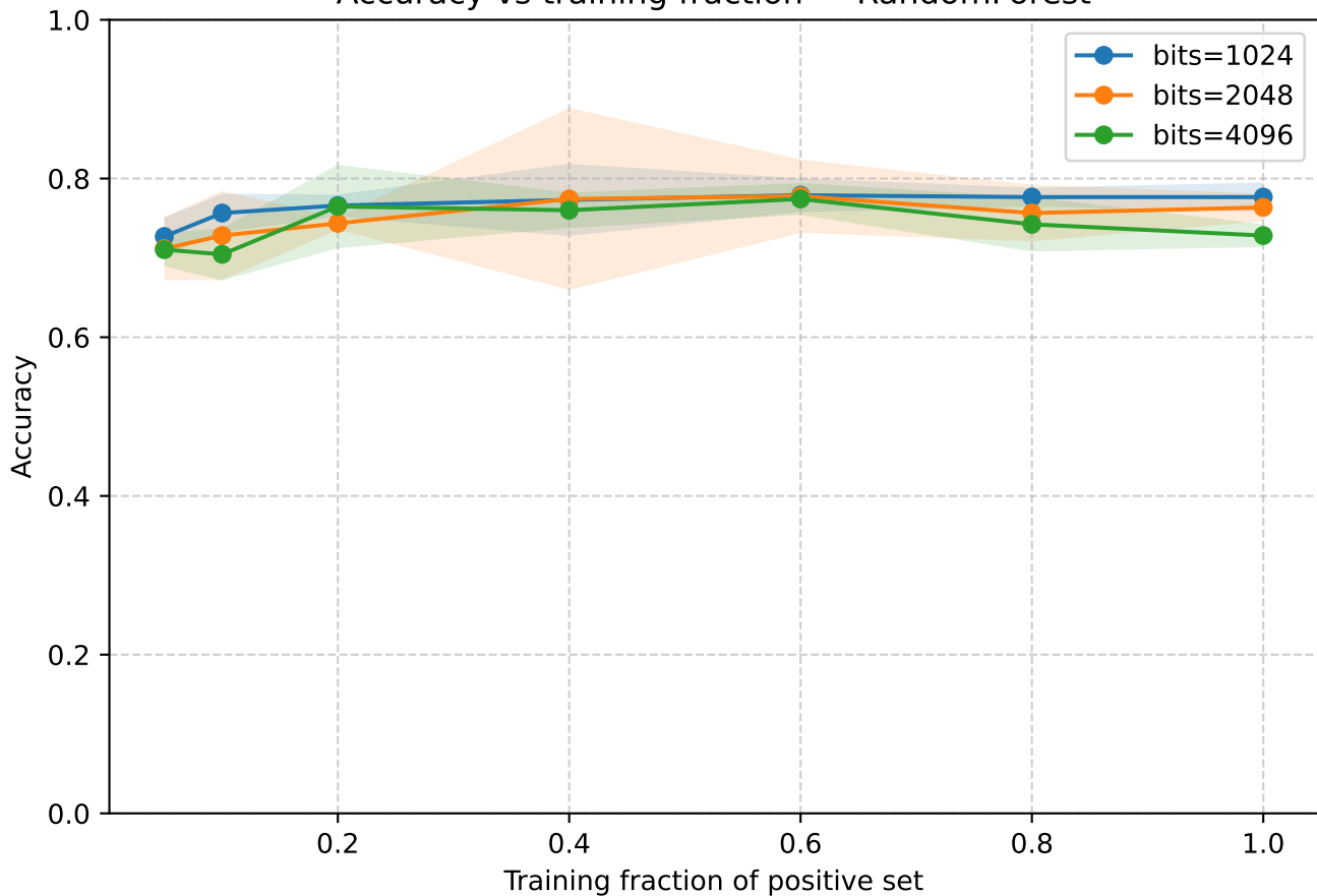
Accuracy vs training fraction — RandomForest
