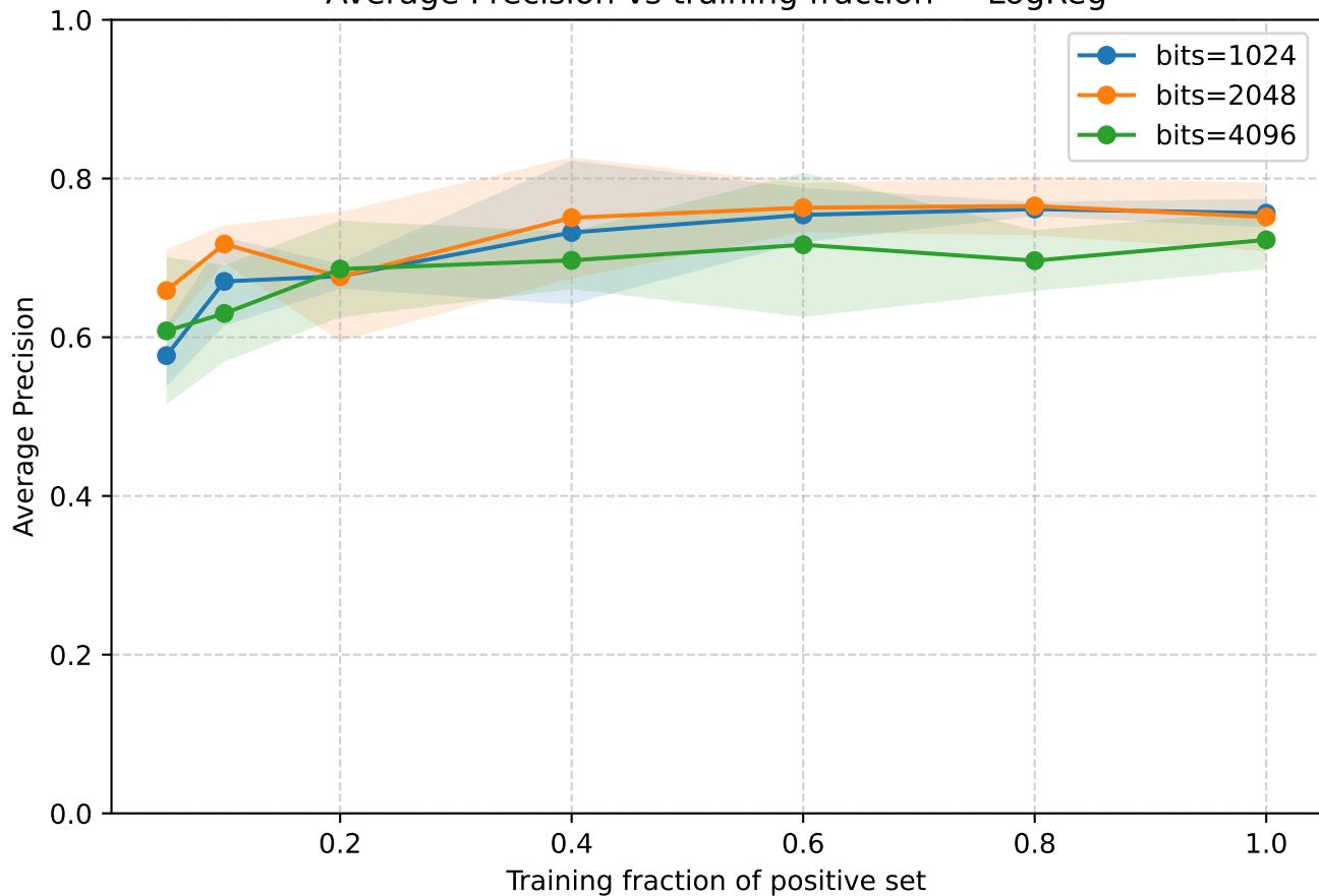
Average Precision vs training fraction — LogReg
