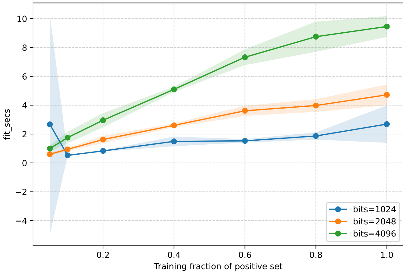
fit_secs vs training fraction — XGBoost
