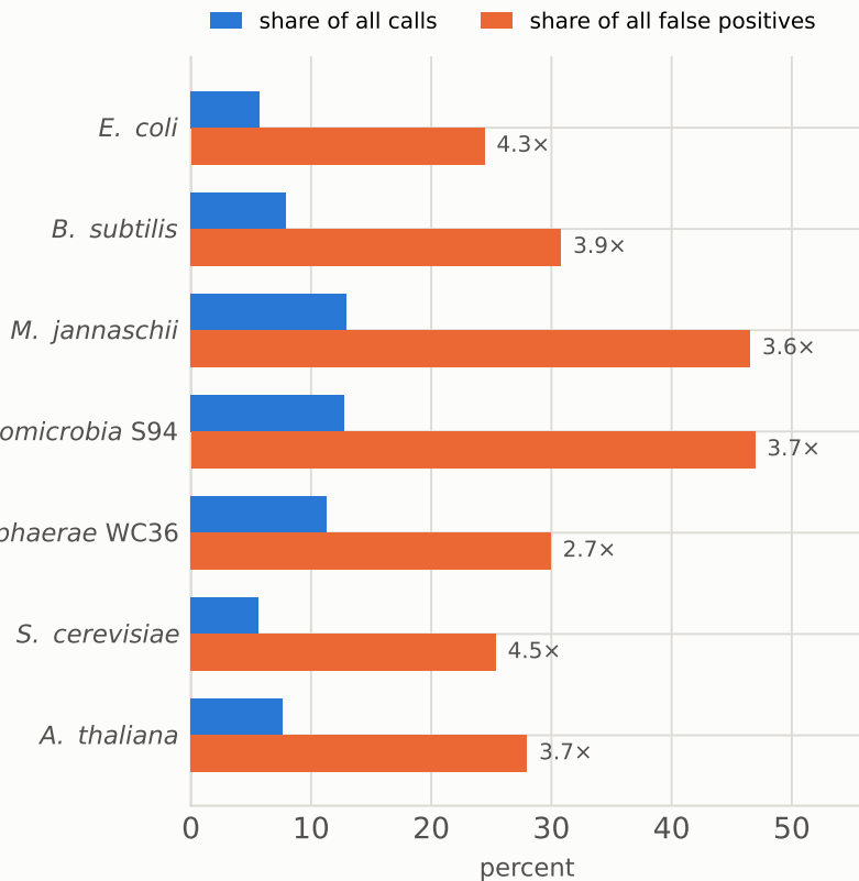
b Calls within 20 bits of threshold
