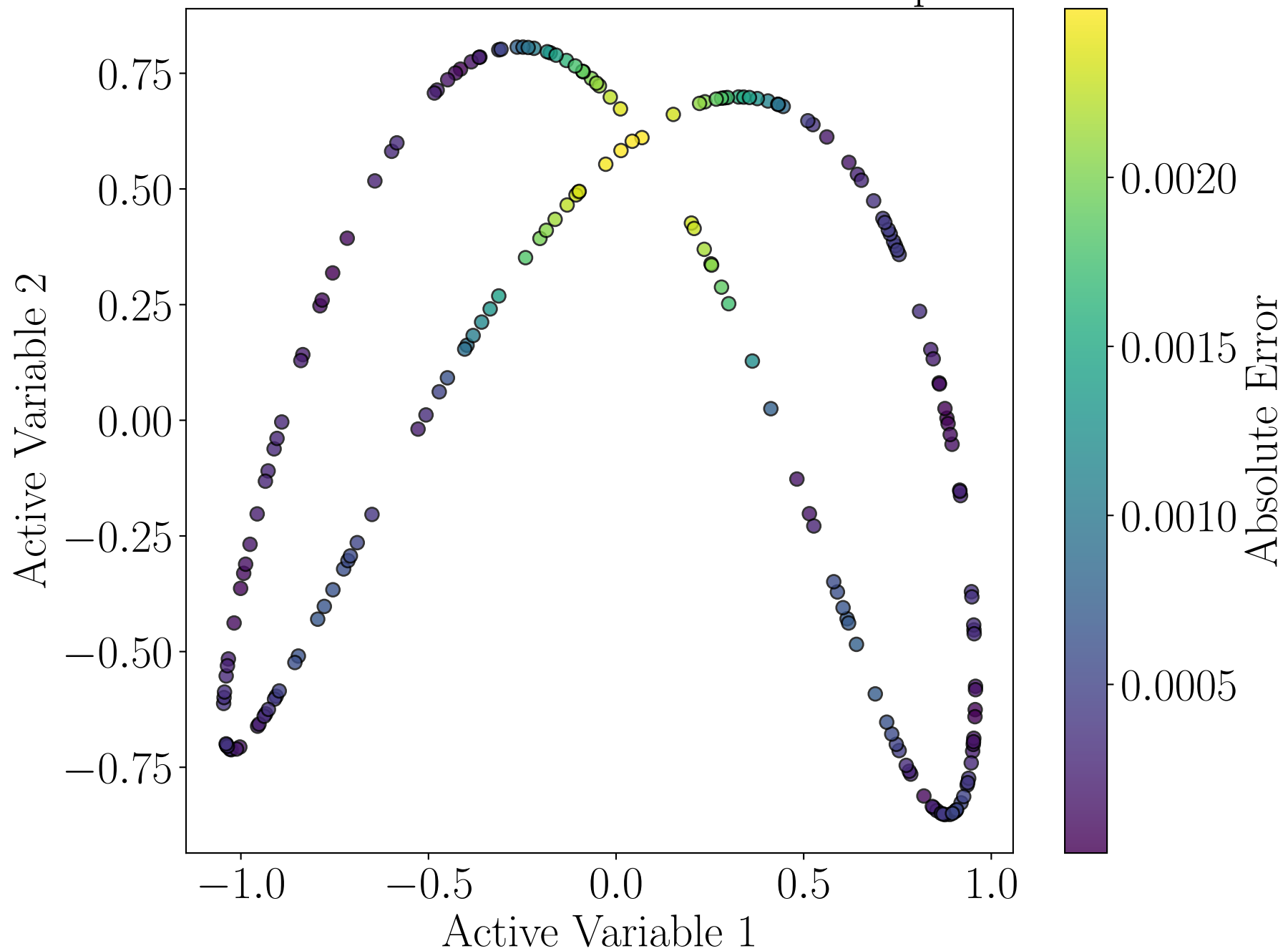
Prediction Error in 2-D Active Subspace
