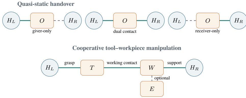
Figure 2: Two complementary topology families. Handover changes which hand supports a shared object; tool-workpiece manipulation introduces a longer, role-asymmetric load path. Dashed edges are inactive or optional.
