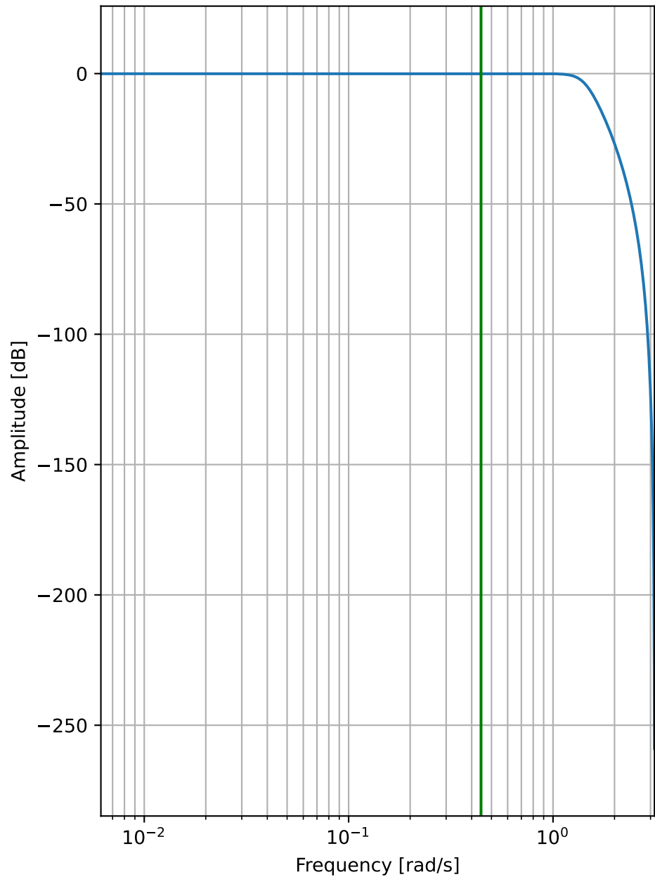
Chebyshev filter frequency response
