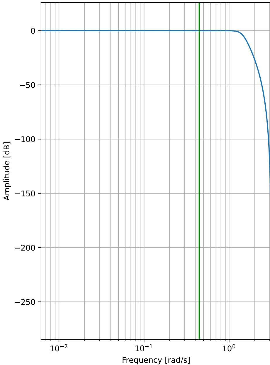
Butterworth filter frequency response
