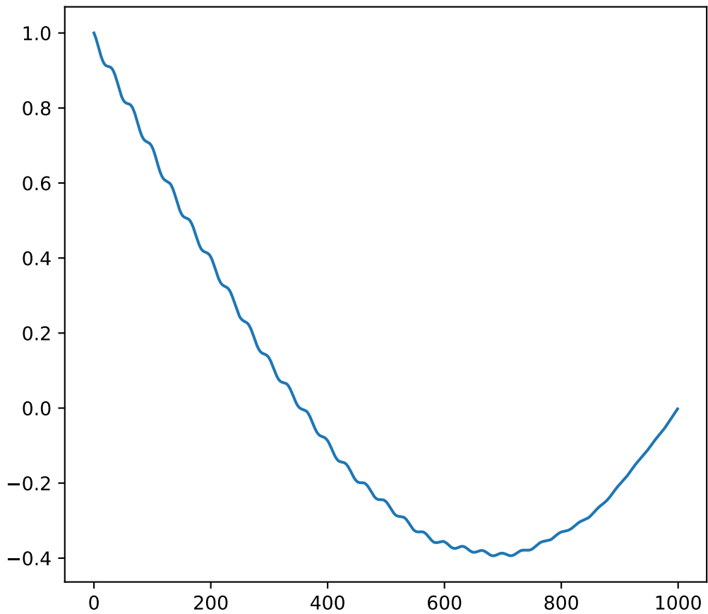
Autocorrelation Pearson
