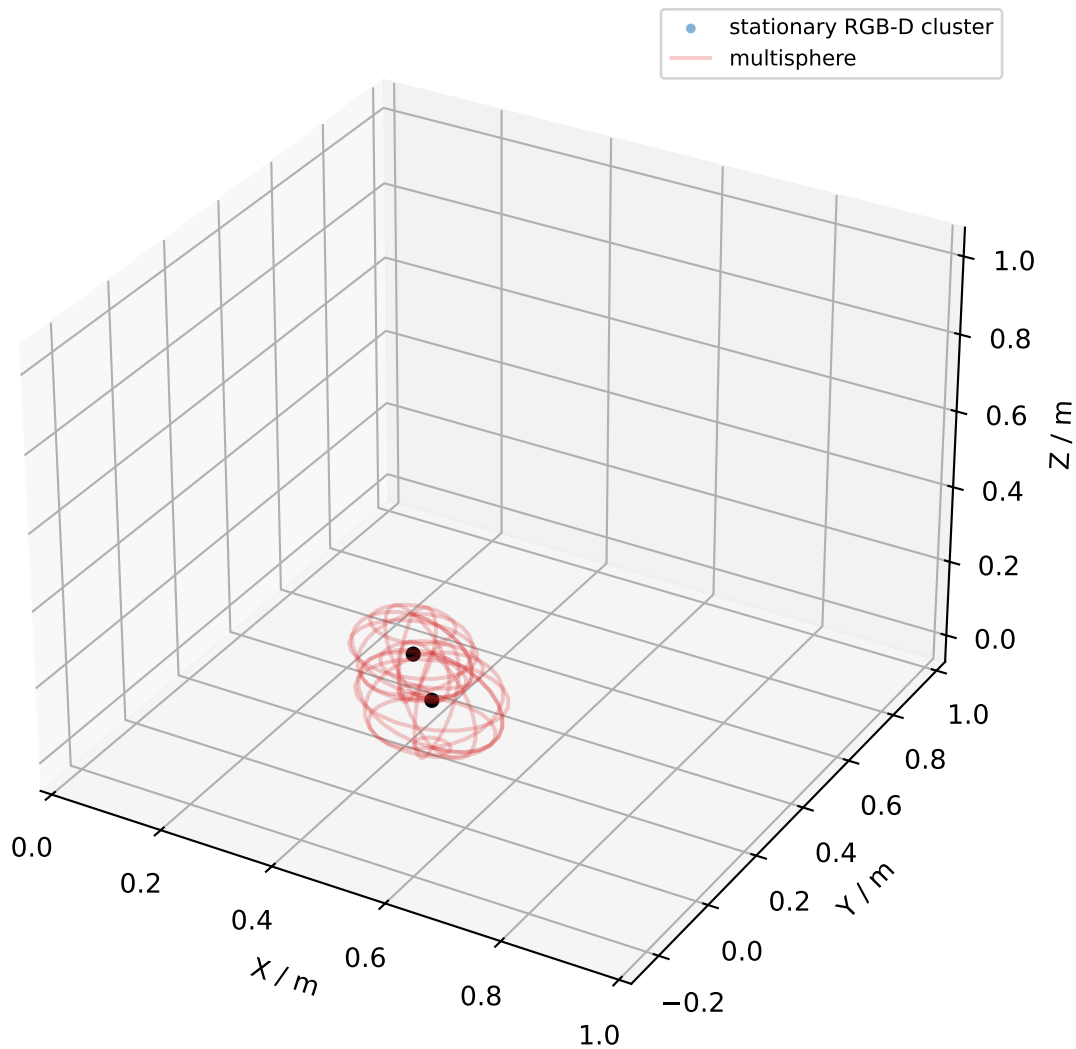
Stationary obstacle point cloud and two-sphere model (r27)
