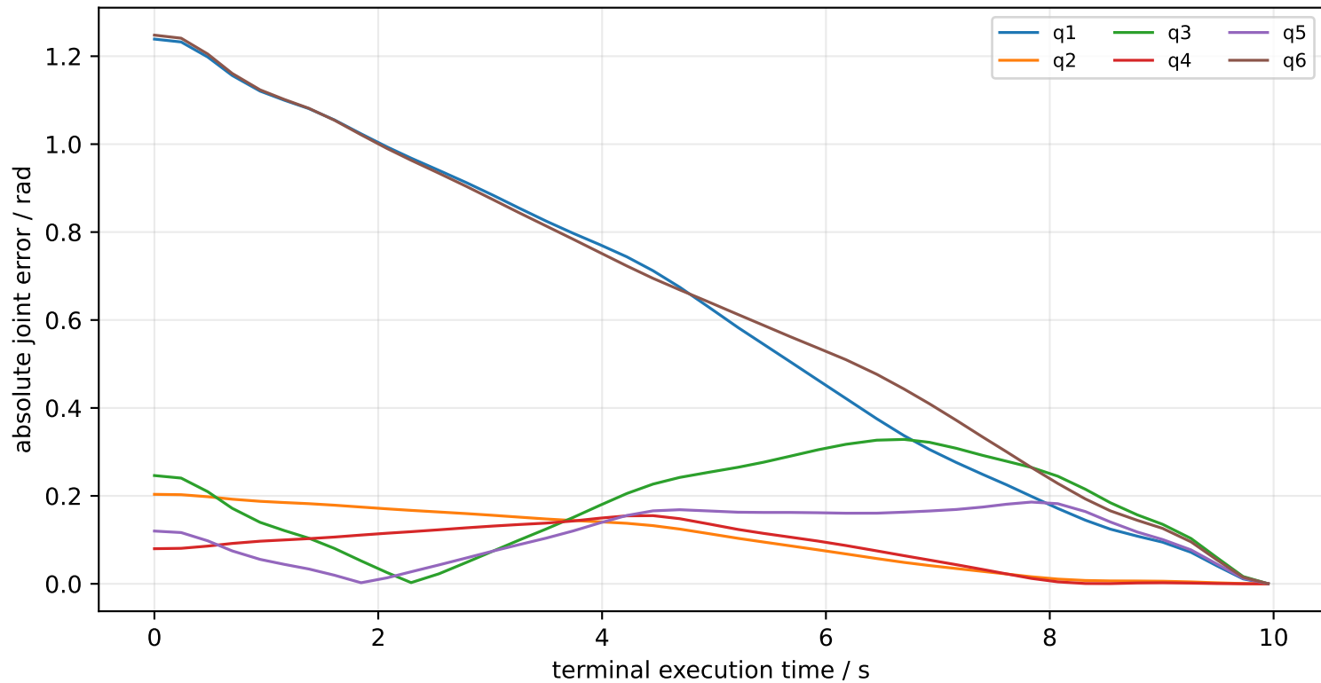
Terminal tracking error (r27)
