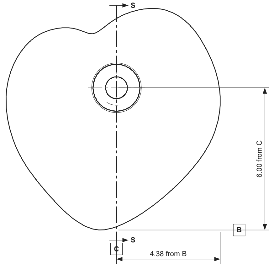
SHELL ALONE / RIGHT SIDE
