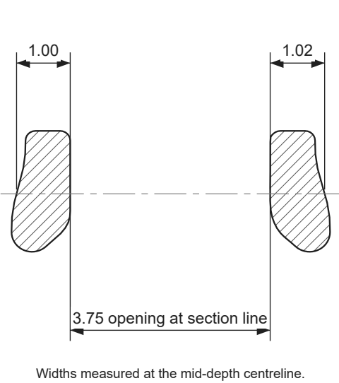
SECTION T-T
