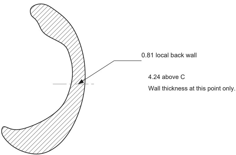
SECTION S-S / THROUGH POST AXIS
