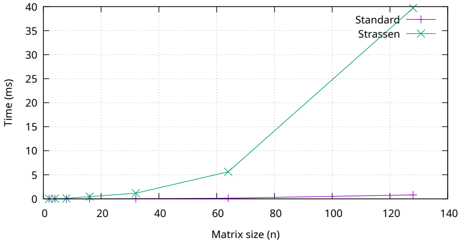
Strassen vs Standard
