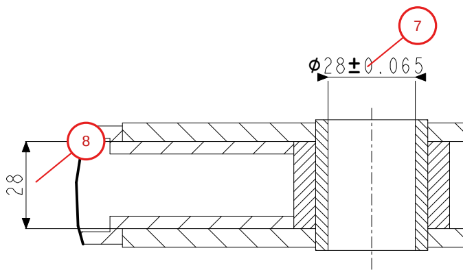
DETAIL B SCALE 0.600
