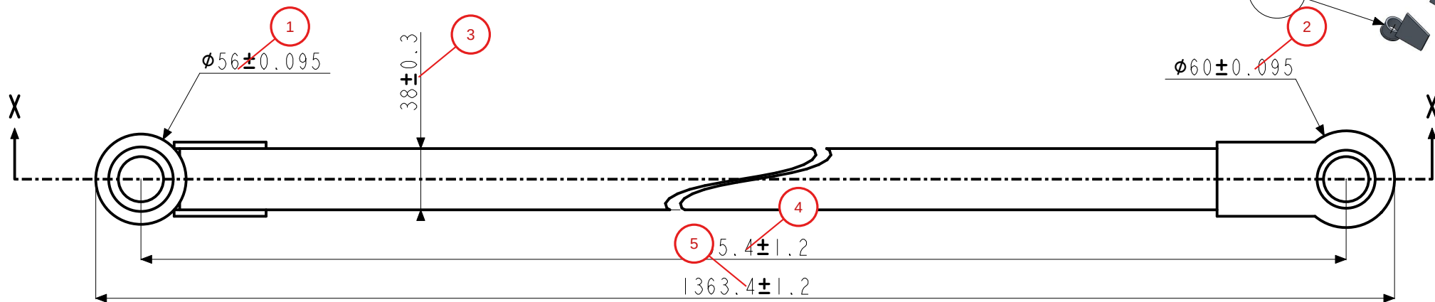
TOP VIEW
