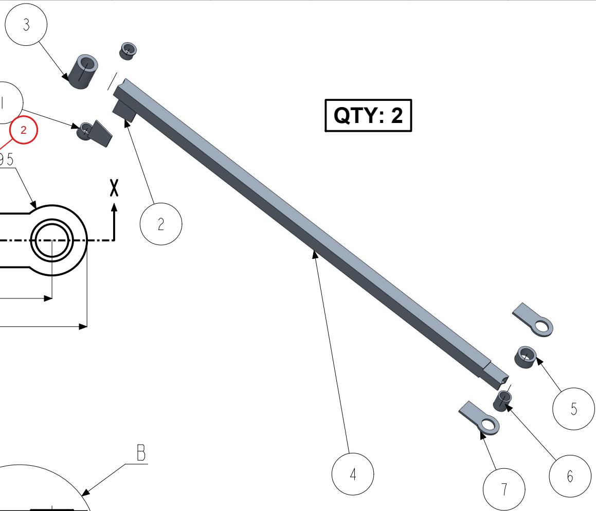
EXPLODED VIEW
