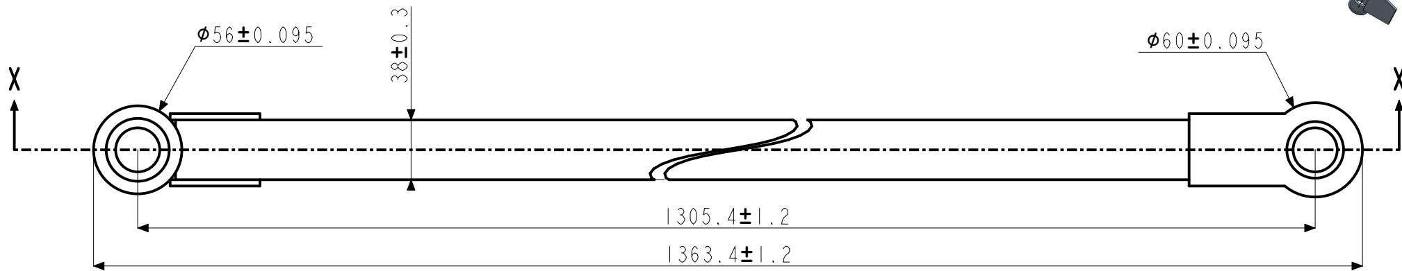
TOP VIEW
