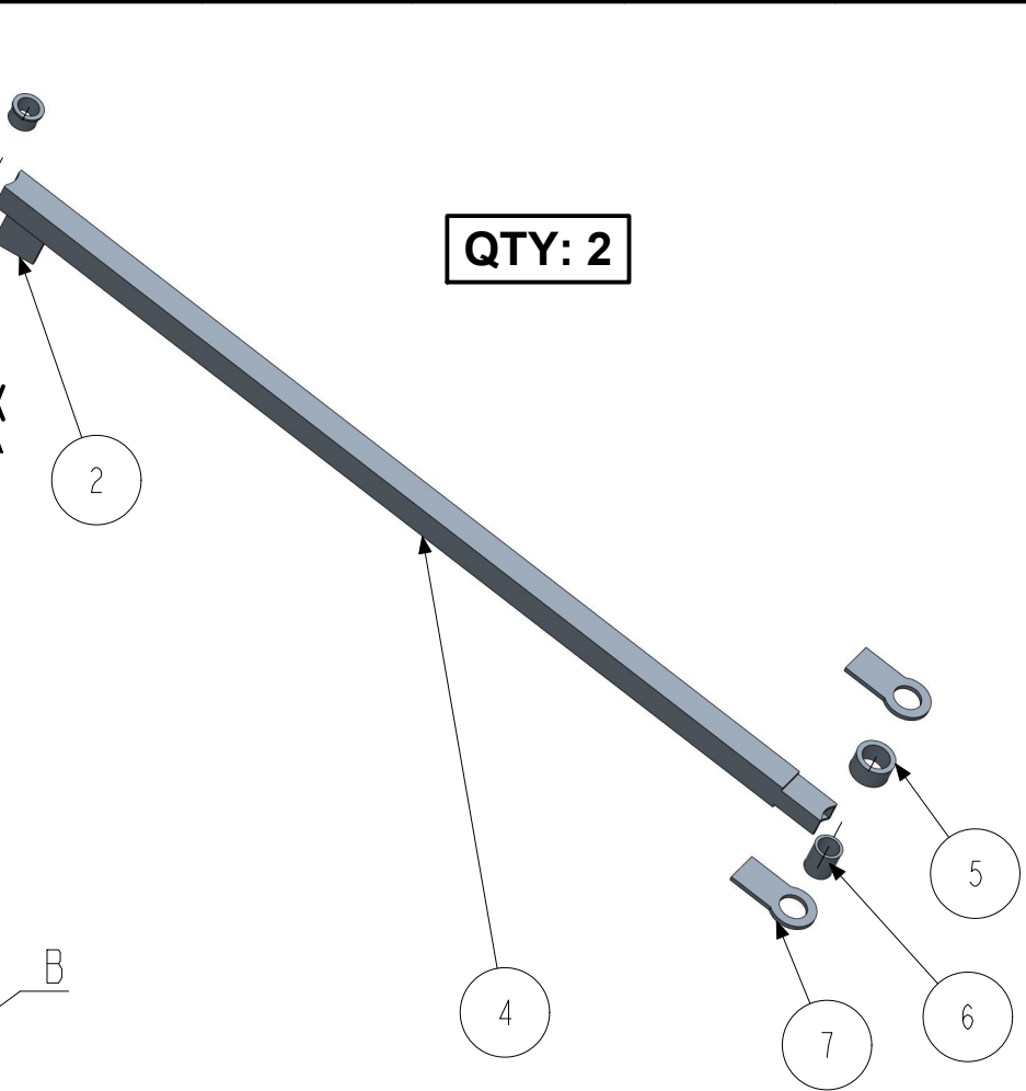
EXPLODED VIEW
