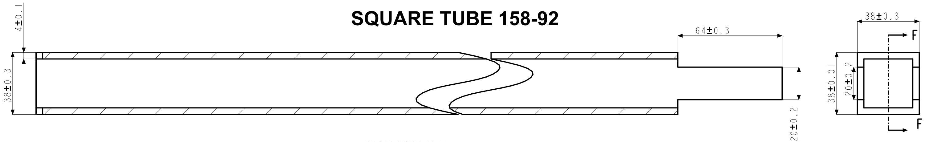
SECTION F-F
