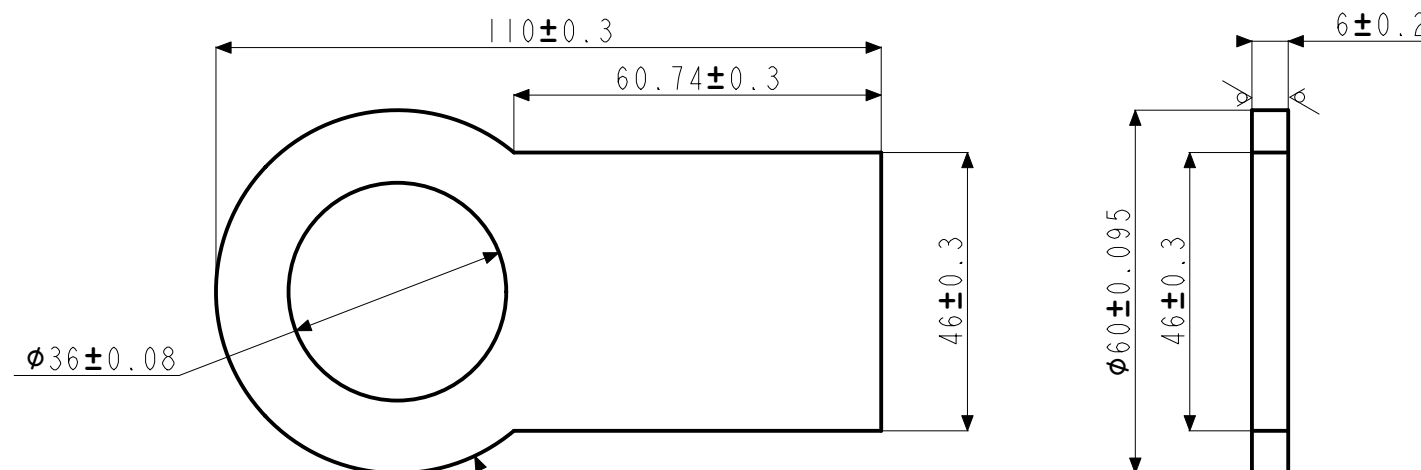
TOP VIEW
