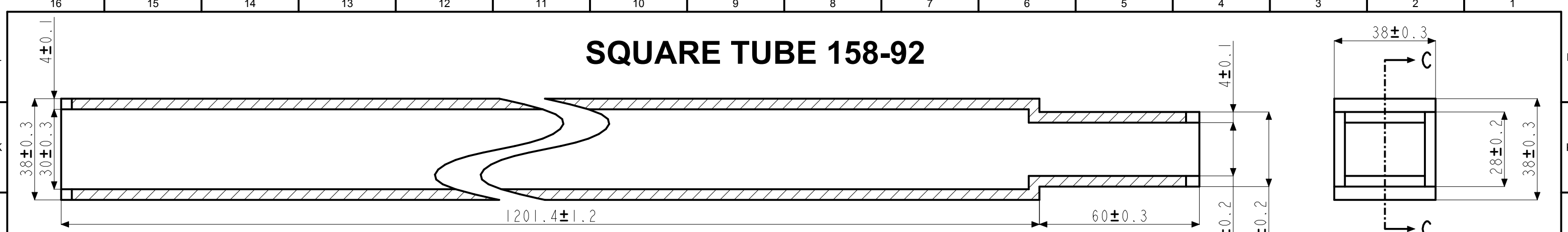
SECTION C-C
