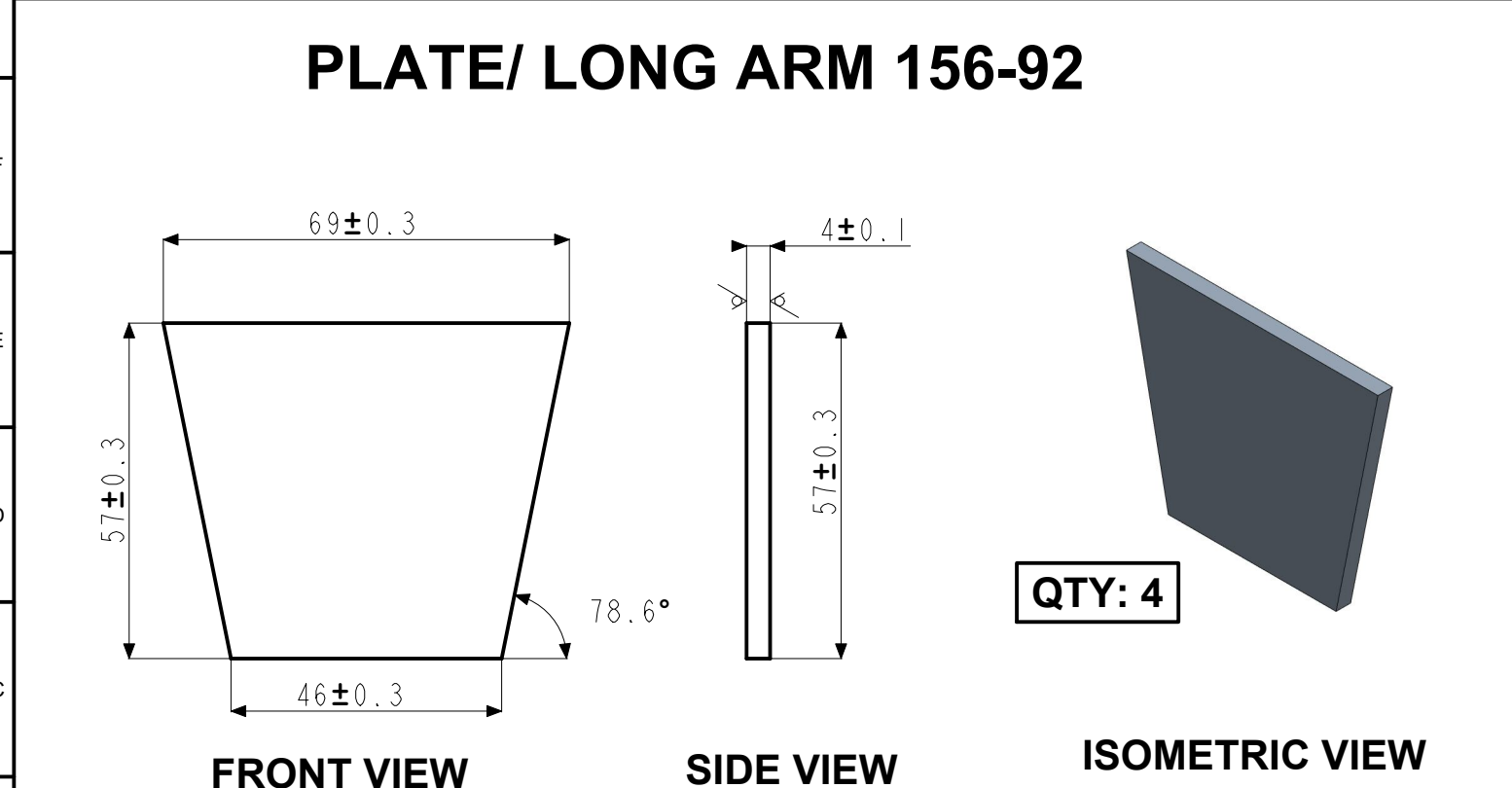
FRONT VIEW
