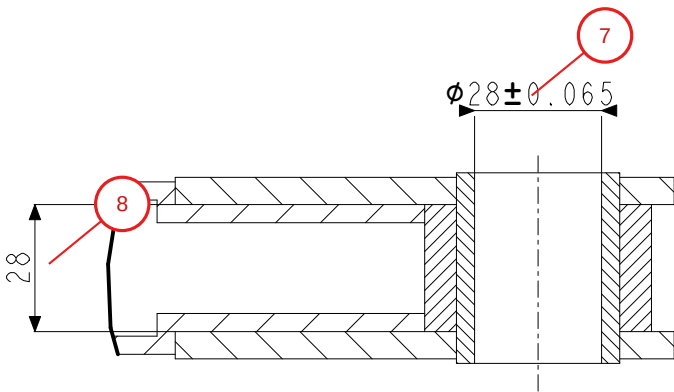
DETAIL B SCALE 0.600
