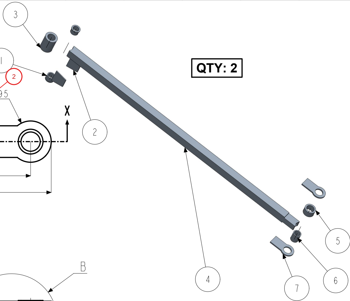
EXPLODED VIEW
