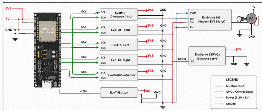
Microcontroller System Diagram (Schematic)
