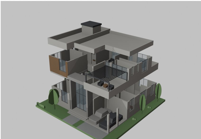
Roof and first floor lifted
