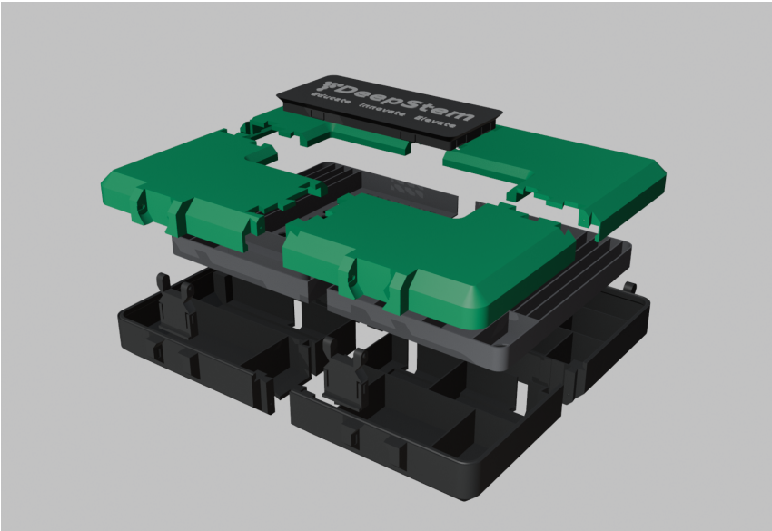
Exploded: 4 base + 4 lid quarters, tray, badge, latches
