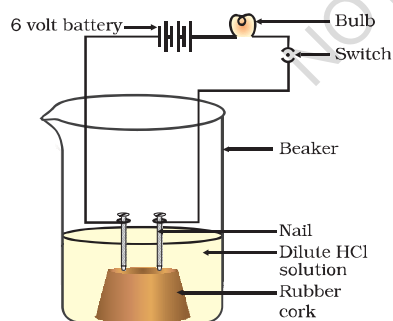
Figure 2.3 Acid solution in water conducts electricity
