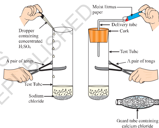
Figure 2.4 Preparation of \text{HCl} gas
