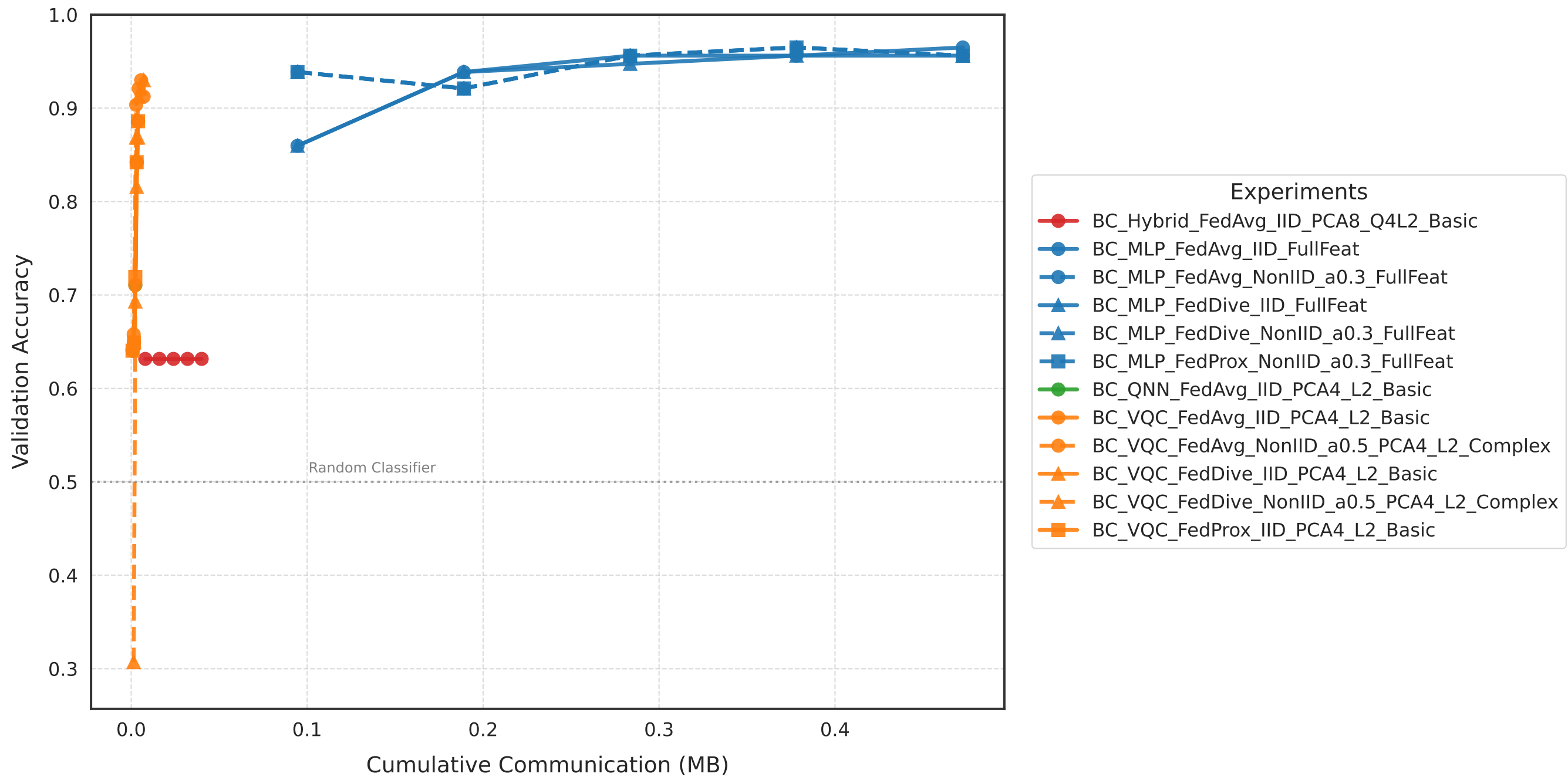
Accuracy vs. Communication Cost
