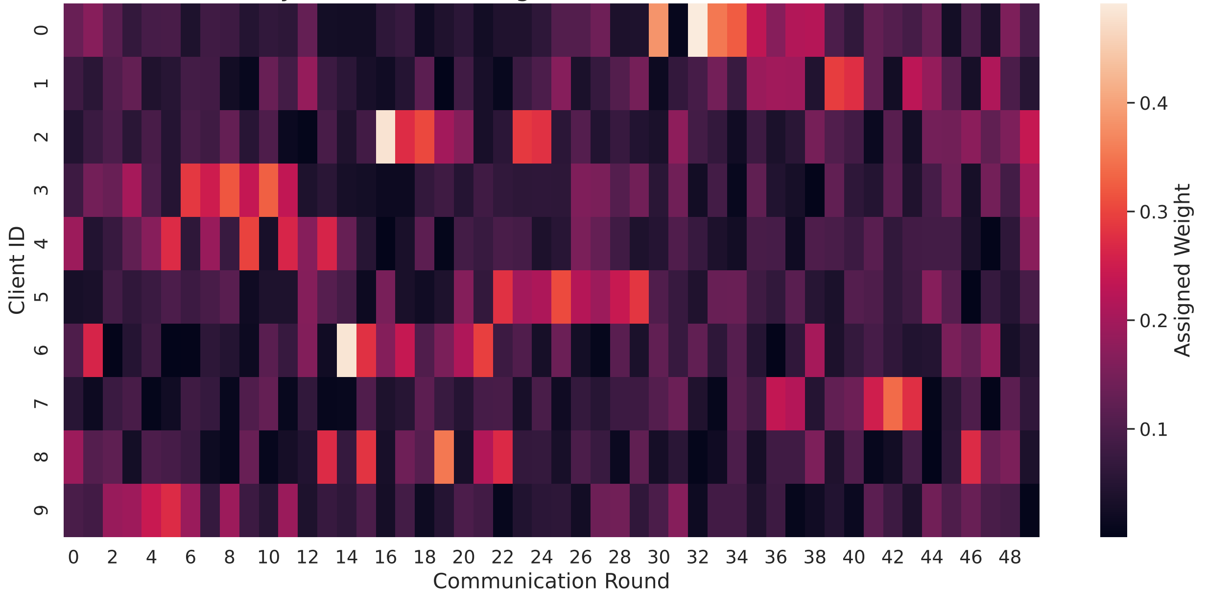
Dynamic Client Weights in FedDive (Non-IID)
