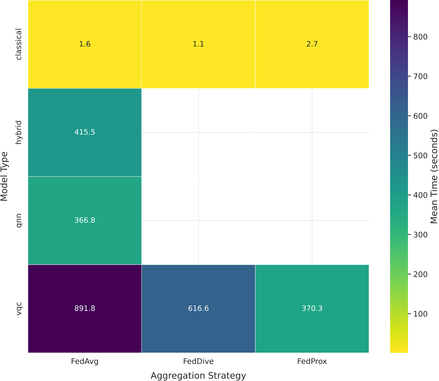
Mean Computation Time by Model Type and Aggregation Strategy
