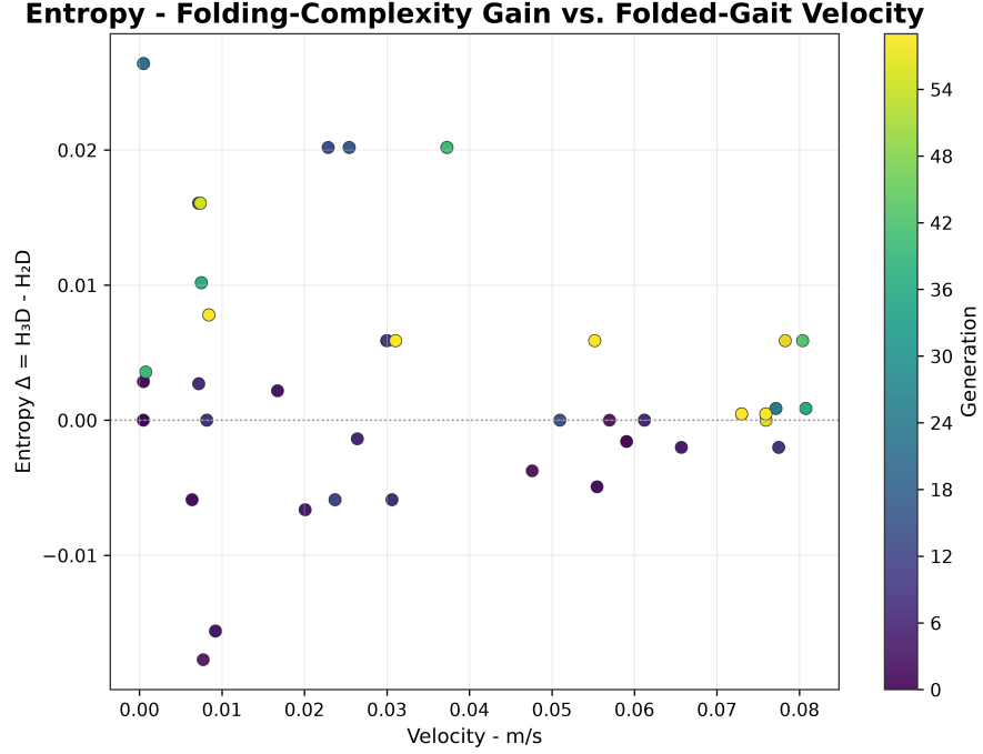
Figure 6.4: Folding-complexity gain ( f_2 = \tilde{H}_{3D} - \tilde{H}_{2D} ) versus folded-gait velocity ( f_1 ), every individual across every generation, coloured by generation.
