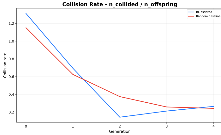
Figure 6.8: Collision rate ( n_{\text{collided}}/n_{\text{offspring}} ), RL-assisted versus random-baseline breeding, over the same preliminary comparison run.
