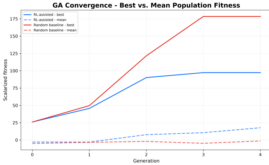
Figure 6.7: Best and mean scalarized fitness, RL-assisted breeding versus the uniform-random baseline (Section 5.2), over a preliminary 5-generation comparison run.
