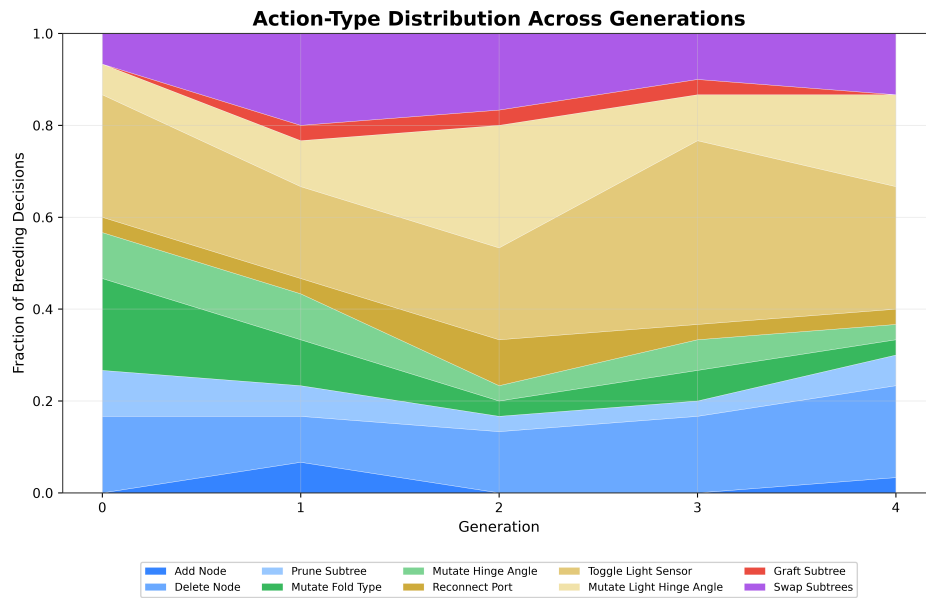
Figure 6.9: Fraction of breeding decisions by grammar action type, per generation.
