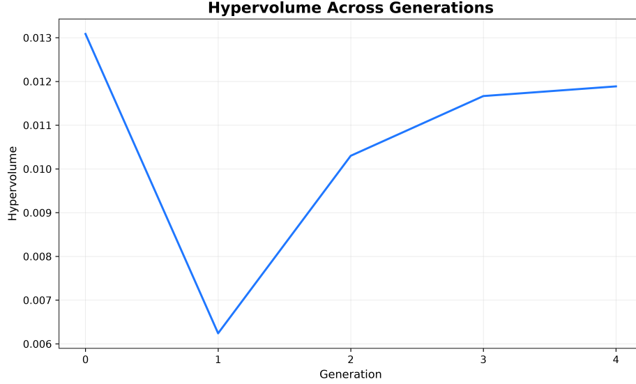
Figure 6.2: Hypervolume of the non-dominated front, per generation, normalized against the run-wide observed objective range (Section 5.3). Rising hypervolume indicates the evolving population’s Pareto front is expanding/improving in aggregate, independent of any single scalarization choice.
