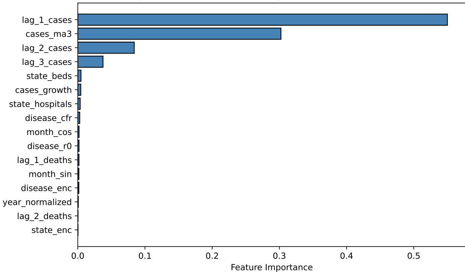
Figure 2: XGBoost Feature Importance — Forecast Model
