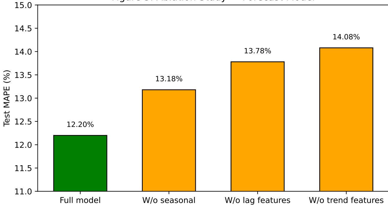
Figure 3: Ablation Study — Forecast Model
