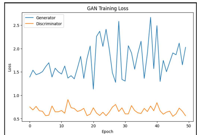
Figure 9: GAN training loss curves for CICIDS2017.
