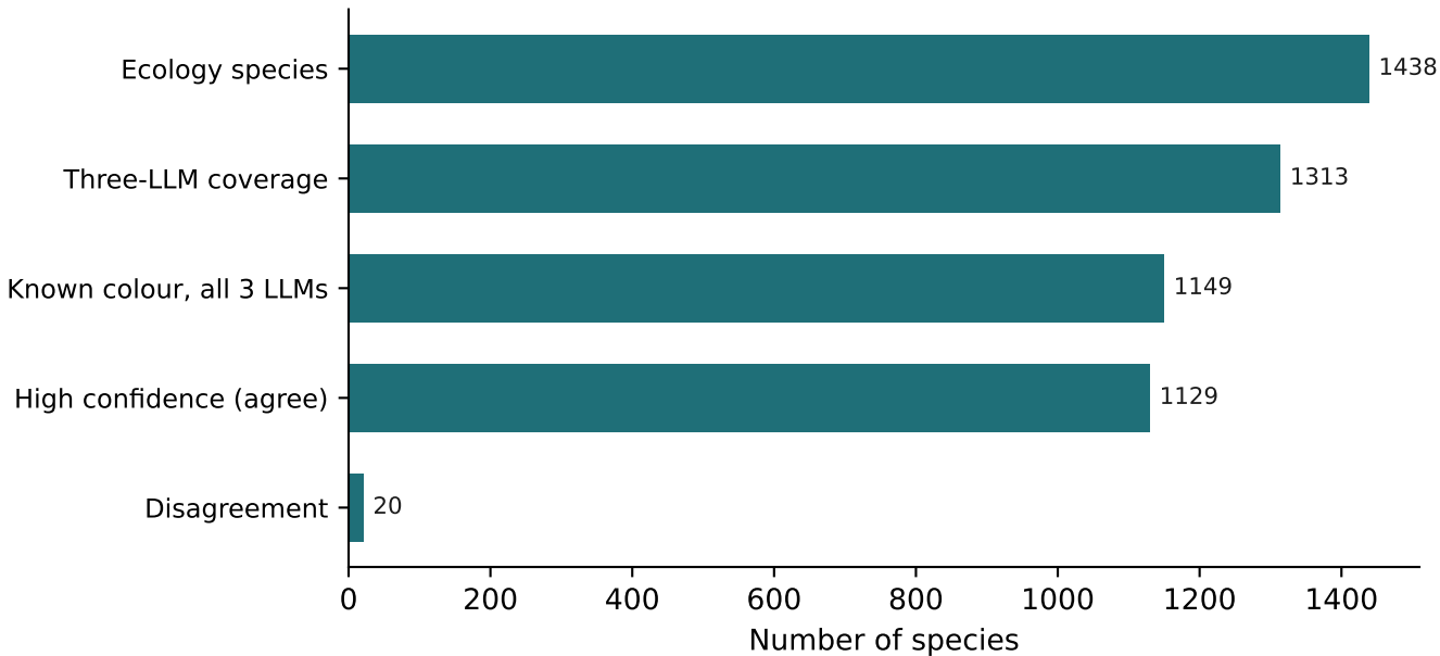
Three-LLM overlap and confidence | unsupported 7B colours: 26
