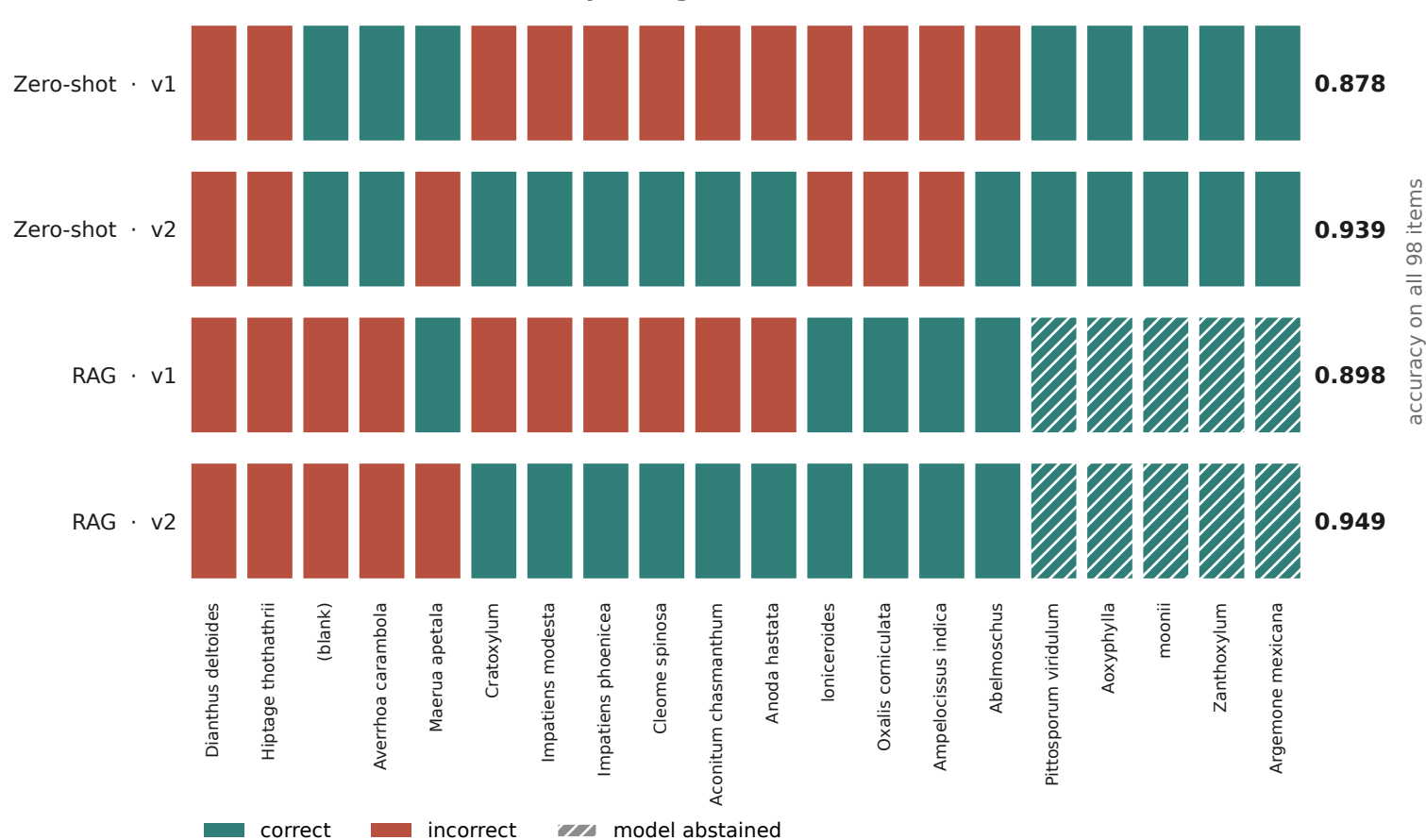
B Qwen2.5-7B · the 20 items any configuration fails or abstains on
