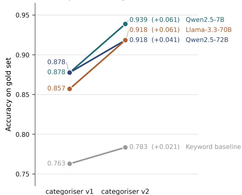
A Accuracy under categoriser v1 and v2
