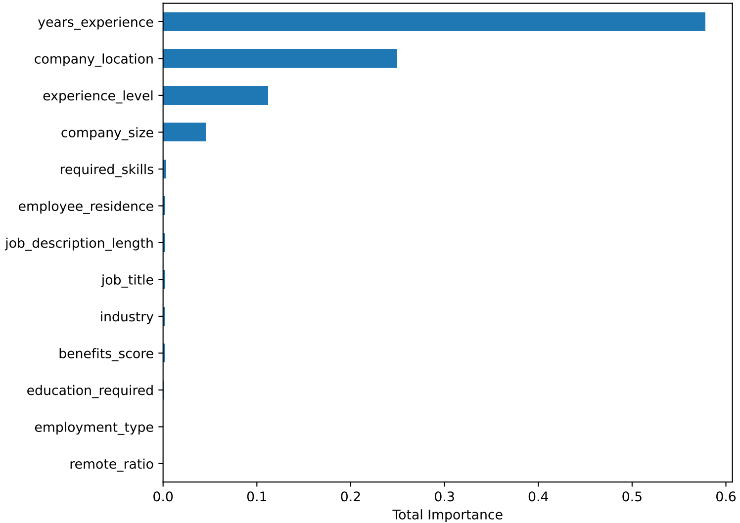
Feature Importances
