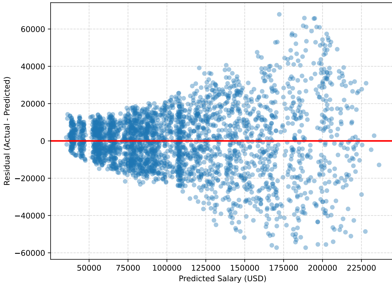
Residuals vs Predicted
