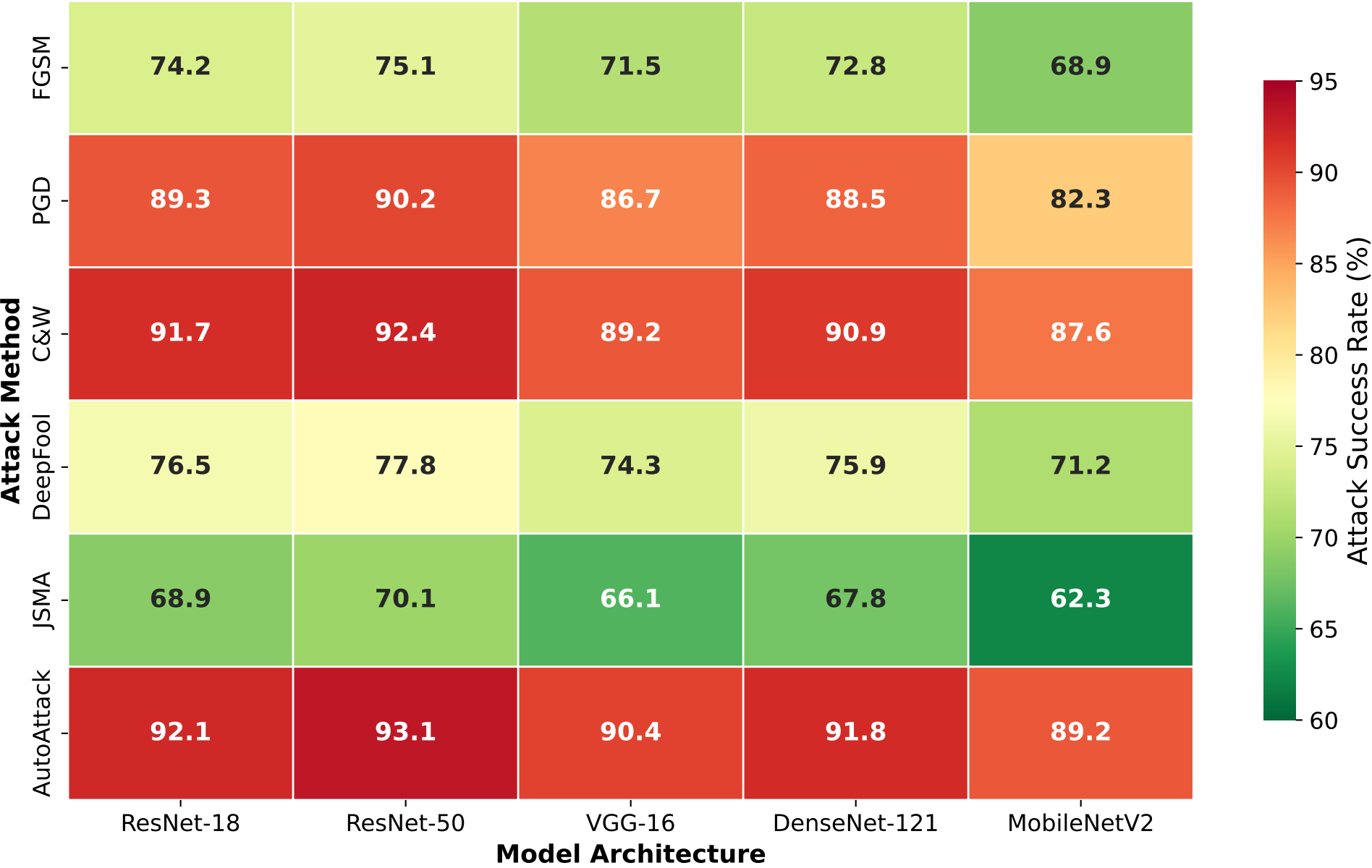
Attack Success Rates (%) at \epsilon=0.03
